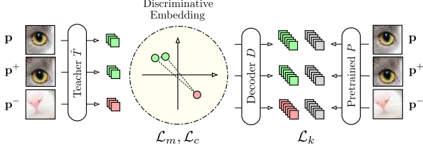
Figure 3: Pretraining of the teacher network \hat{T} to output descriptive embedding vectors for patch-sized inputs. The knowledge of a powerful but computationally inefficient network P is distilled into \hat{T} by decoding the latent vectors to match the descriptors of P . We also experiment with embeddings obtained using self-supervised metric learning techniques based on triplet learning. Information within each feature dimension is maximized by decorrelating the feature dimensions within a minibatch.
