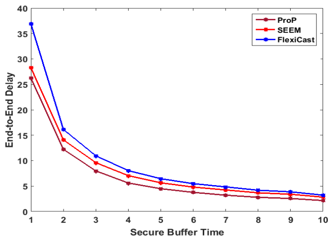
Fig. 3. Comparative Analysis of End-To-End Delay.
