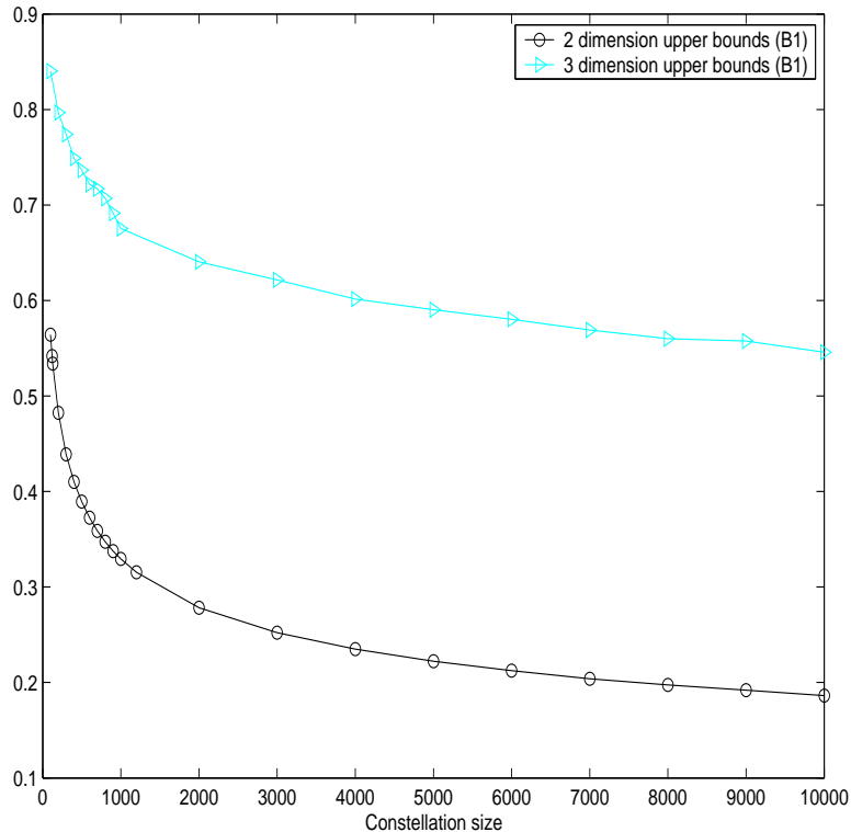
Figure 2: Upper bounds for 2 and 3 dimensional constellations
