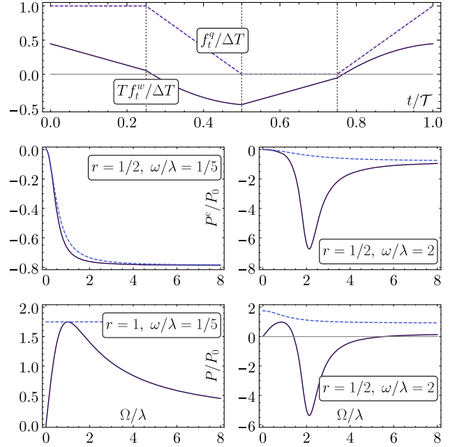
FIG. 2. Single-qubit engine. (Upper panel) The temperature profile f_t^q (dashed line) consists of two isothermal steps at temperatures T + \Delta T and T connected by linear slopes. The work protocol f_t^w (solid line) is determined by the condition (25). (Lower panels) Coherent and total power (solid lines) in units of P_0 \equiv (\hbar\omega\lambda/2)(\Delta T/T)^2 10^{-2} as functions of the rescaled frequency \Omega/\lambda . The bounds (24) are shown for comparison (dashed lines). The plots in the left column show that our bounds (15) and (17) can be practically saturated for \omega/\lambda \ll 1 . For \omega/\lambda > 1 , coherence-induced features (resonant dips) appear in both P^c and P ; see the right column. For all plots, we have set \kappa \equiv 1 .
