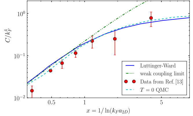
FIG. 5 (color online). Contact density C vs interaction strength 1/\ln(k_F a_{2D}) at temperature T/T_F = 0.27 . We compare our result (blue solid line) with the experimental data at T/T_F = 0.27 [13] (red symbols), the weak-coupling result (green dashed-dotted line), and QMC calculations at T = 0 [11] (cyan dashed line).
