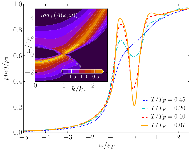
FIG. 1 (color online). Density of states \rho(\omega) , normalized by \rho_0 = m/2\pi for the free Fermi gas, at interaction \ln(k_F a_{2D}) = 0.8 for different temperatures: T = 0.45T_F (top curve at \omega = 0 ) to T = 0.07T_F (bottom). Inset : Spectral function A(k, \omega) for T = 0.07T_F . The grey dashed line marks the maximum in the spectral weight of the bottom band.
