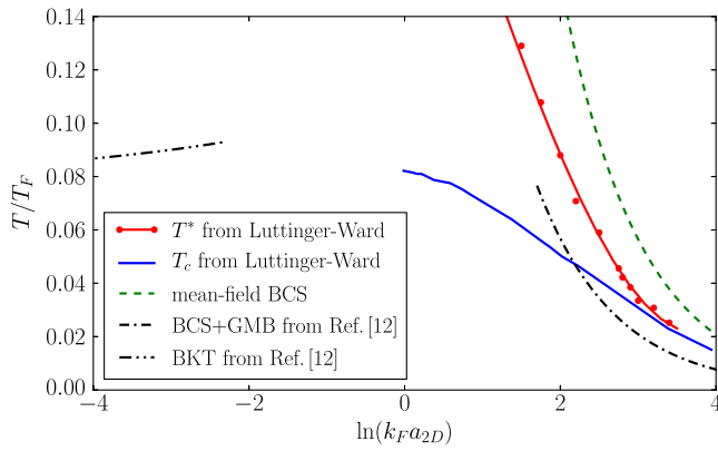
FIG. 4 (color online). Critical temperature T_c/T_F vs interaction strength \ln(k_F a_{2D}) . The Luttinger-Ward result for a finite system (blue solid line) in the crossover region \ln(k_F a_{2D}) \gtrsim 0 is compared with analytical limits [12]. The red dots mark the crossover temperature T^* to the pseudogap regime for \ln(k_F a_{2D}) \gtrsim 1 .
