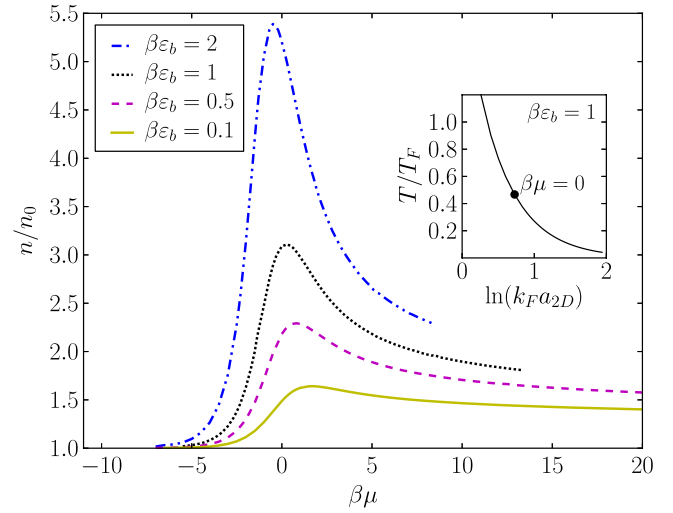
FIG. 2 (color online). Density n of the 2D Fermi gas vs chemical potential \beta\mu , for different interaction strengths \beta\varepsilon_B (see legend). Since the density is normalized by n_0(\beta\mu) for the noninteracting gas, the nonmonotonic behavior of n/n_0 reflects the impact of interactions, while the compressibility \kappa = (\partial n / \partial \mu) / n^2 is always positive. The inset shows a typical trajectory in T/T_F vs \ln(k_F a_{2D}) corresponding to the dotted line of fixed \beta\varepsilon_B = 1 . Along this line, \beta\mu increases with decreasing T/T_F .
