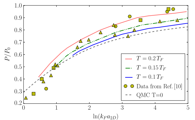
FIG. 3 (color online). Pressure P vs interaction strength, normalized by the pressure P_0 = n\varepsilon_F/2 of an ideal Fermi gas of the same density at T = 0 . Luttinger-Ward data at temperature T/T_F = 0.2 (top, dotted line) to T/T_F = 0.1 (solid line) in comparison with experimental data [10] (symbols) and T = 0 QMC results [11] (dashed line).
