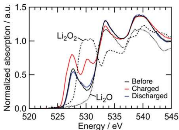
Fig. 4 O K-edge XANES spectra of NiDL cathode during charge/discharge.
