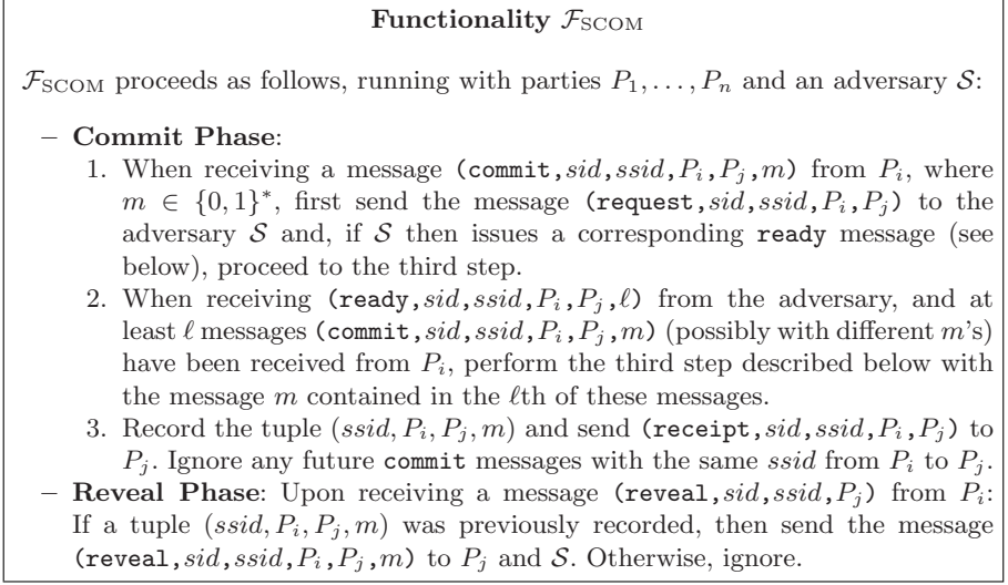
Fig. 2. Functionality \mathcal{F}_{\text{SCOM}}
