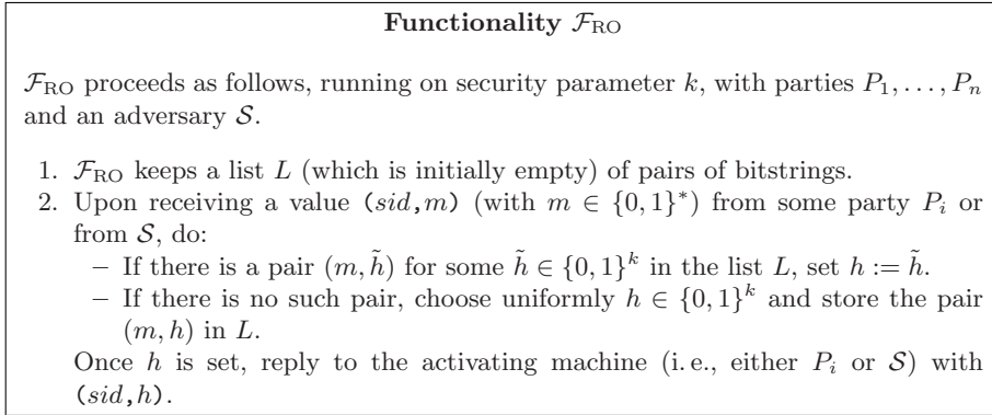
Fig. 1. Functionality \mathcal{F}_{\text{RO}}
