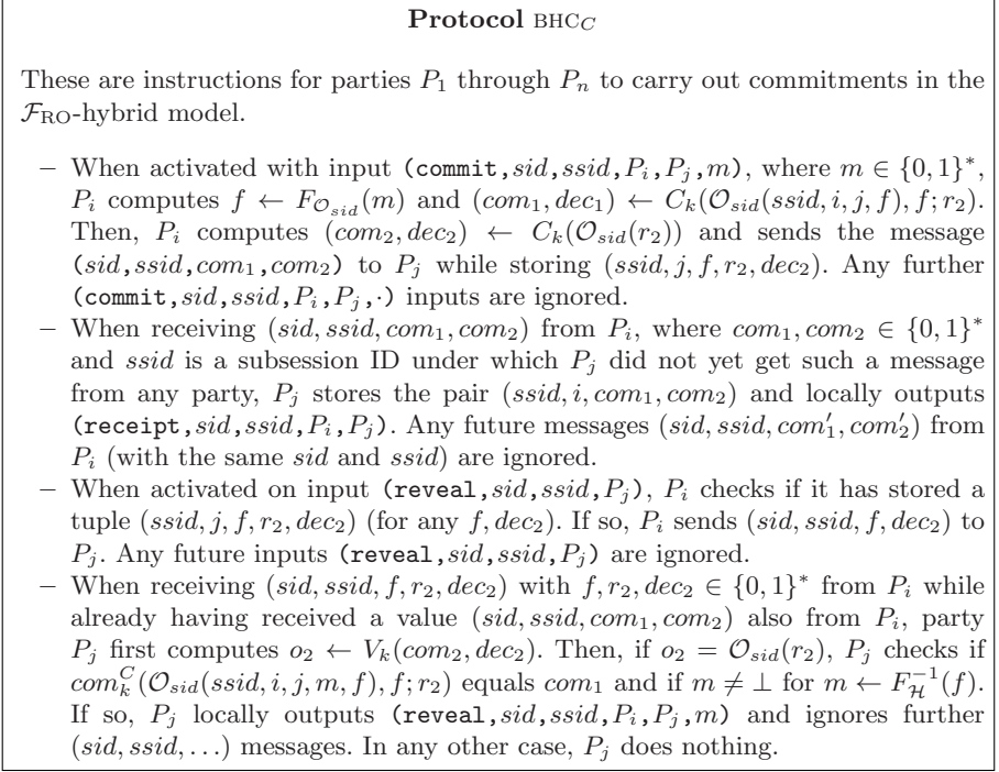
Fig. 4. Protocol \text{BHC}_C
