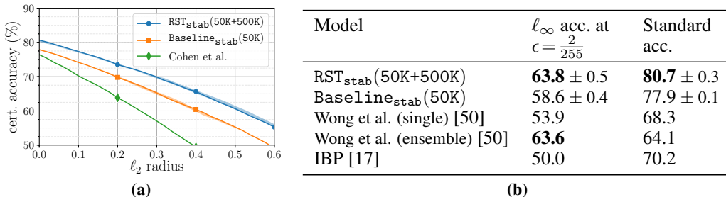
Figure 1: Certified defense. Guaranteed CIFAR-10 test accuracy under all \ell_2 and \ell_\infty attacks. Stability-based robust self-training with 500K unlabeled Tiny Images (RST stab (50K+500K)) outperforms stability training with only labeled data (Baseline stab (50K)). (a) Accuracy vs. \ell_2 radius, certified via randomized smoothing [9]. Shaded regions indicate variation across 3 runs. Accuracy at \ell_2 radius 0.435 implies accuracy at \ell_\infty radius 2/255 . (b) The implied \ell_\infty certified accuracy is comparable to the state-of-the-art in methods that directly target \ell_\infty robustness.
