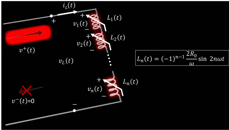
FIG. 4. Transmission line terminated by an infinite number of time-dependent inductances connected in series.
