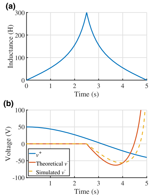
FIG. 2. (a) Time-modulated inductance, as the load of the transmission line, in the accumulation and release regimes. (b) The incident and reflected waves (simulated and theoretical) at the load position. Here R_0 = 50 \Omega and v^+(t) = 50 \cos \omega t V, where \omega = 0.5 rad/s.
