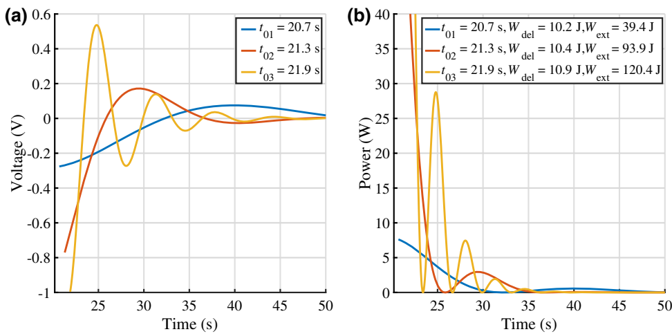
FIG. 8. (a) The resistance voltage and (b) the corresponding instantaneous power consumed by the resistance ( R = 0.01 \Omega ) after the time modulation is stopped at different moments. Here R_0 = 1 \Omega , \omega = 1 rad/s, A = 1 V, and I_0 = 1 A/s.
