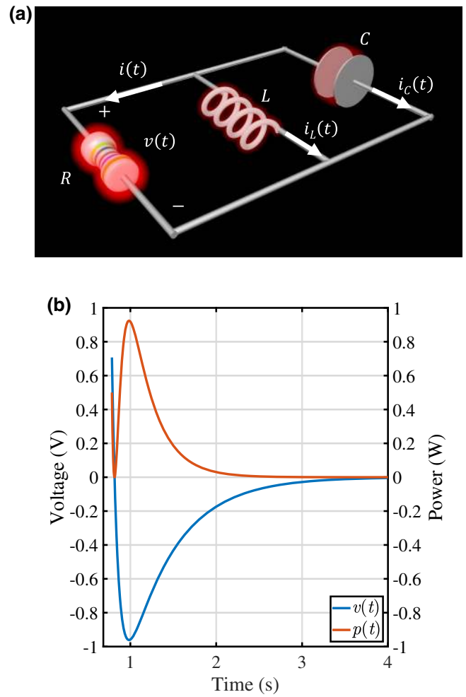
FIG. 6. (a) The corresponding RLC circuit after the stopping of temporal modulation. (b) The instantaneous voltage and the power consumed by the resistance R = 1 \Omega . Here t_0 = \pi/4\omega , \omega = 1 \text{ rad/s} , R_0 = 1 \Omega , A = 1 \text{ V} , and I_0 = 1 \text{ A/s} .
