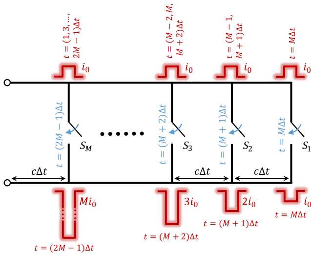
FIG. 3. Space-time-modulated transmission line with M switches. Each switch is closed at specific moments shown in blue. The amplitudes of the signal at different locations of the transmission line at different moments are depicted in red.
