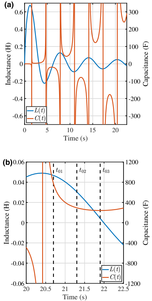
FIG. 7. Time-dependent inductance and capacitance for R_0 = 1 \Omega , \omega = 1 \text{ rad/s} , A = 1 \text{ V} , and I_0 = 1 \text{ A/s} .
