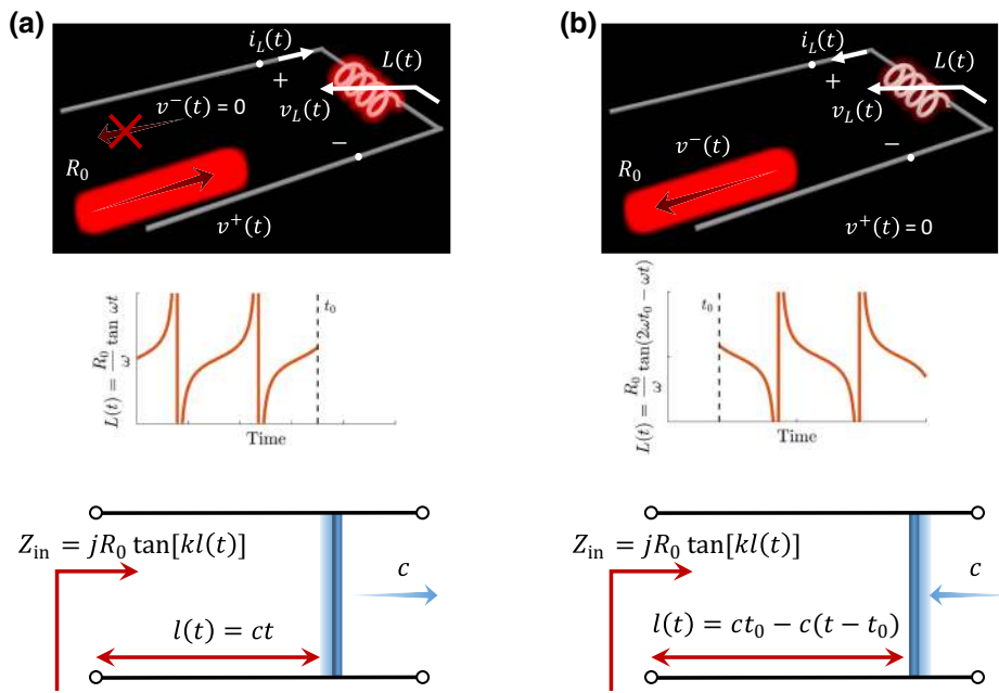
FIG. 1. (a) Transmission line terminated by a time-dependent inductance that absorbs the incoming energy. The white arrow depicted on the time-varying inductance shows that this element is active and contains an internal modulation source that varies the inductance in time. The bottom illustration shows its conceptual realization by a short-circuited line whose length increases with a constant velocity. (b) Energy release by the same line but with different inductance modulation (inverse with respect to moment t_0 ). This means that in its conceptual realization, the load is moving in the opposite direction.
