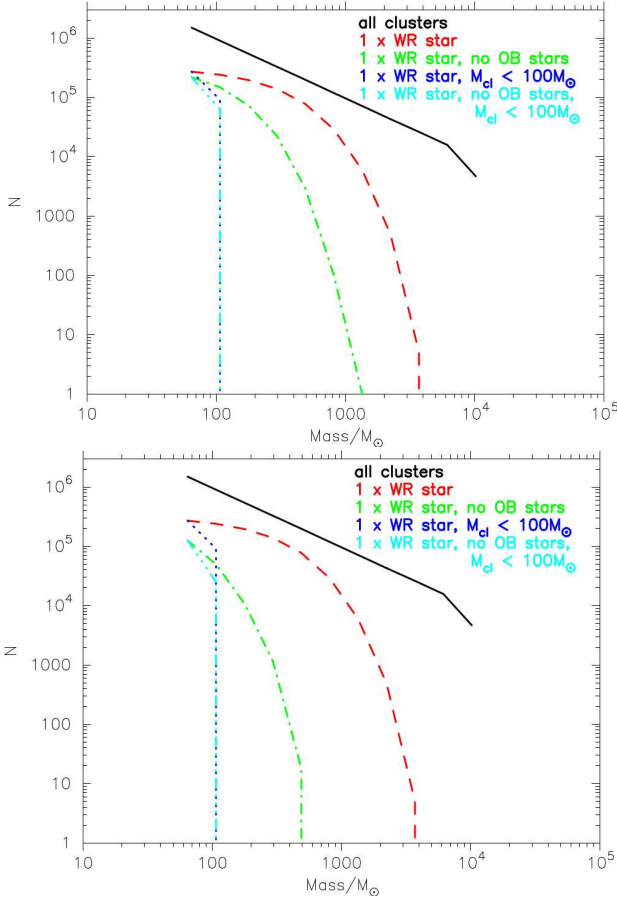
Figure 3. Monte Carlo simulations of the number of clusters with different masses, which contain WR stars. Each line shows the relation between cluster mass and number if they contain one WR star. The cutoff applied in the upper panel was >10 M_{\odot} to OB stars (corresponding to O stars and early B stars, which are the brightest OB subtypes) and >25 M_{\odot} for WR stars. For the lower panel the cutoff was >5 M_{\odot} for OB stars (a stricter criterion removing O stars, early B and mid B stars) and >25 M_{\odot} for WR stars.
