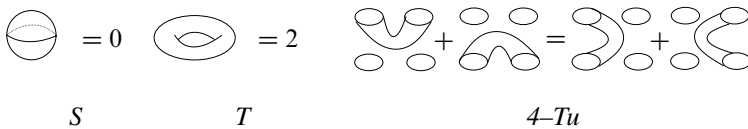
Figure 5: Bar-Natan's relations
