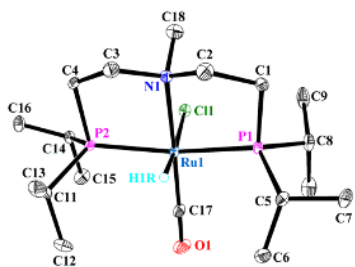
Figure 2. ORTEP view of anti Me-1a with thermal ellipsoids drawn at the 30% probability level. H atoms (except HiR) are omitted for clarity.
