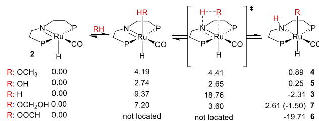
Scheme 7. B 3 PW 9 I-generated Gibbs free-energies (kcal mol -1 ) of protic species addition to Ru-amido complex 2 . P = Pi-Pr 2 .
