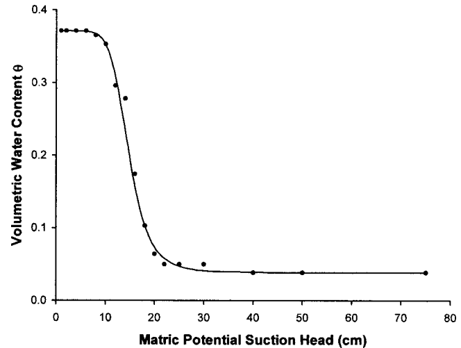
Fig. 1. Drying loop of the water characteristic curve. Circles are data points and curve is best fit of Eq. [3].
