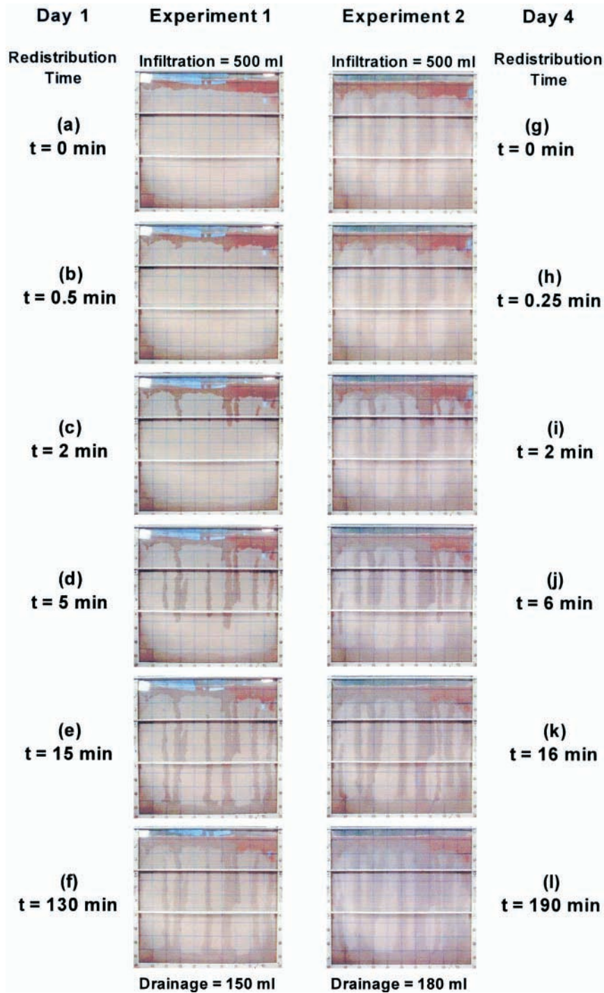
Fig. 2. Photographs of the wetting front taken at different times (a–f) during redistribution in dry sand and (g–l) during second cycle of redistribution with fingers in the sand. The redistribution time is indexed from t = 0 , defined as the moment when ponded water first disappeared from the sand surface.
