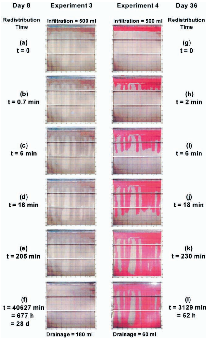
Fig. 3. Wetting front patterns (a-f) during the third cycle of redistribution with fingers in the sand and (g-l) during the fourth cycle of redistribution with diffused fingers in the sand.
