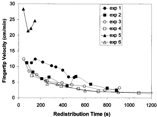
Fig. 6. Wetting front speed during ponded infiltration (Exp. 5) and redistribution in other experiments.
