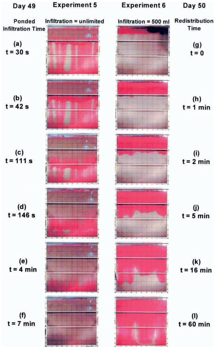
Fig. 5. Wetting front patterns (a-f) during ponded infiltration with fingers in the sand and (g-l) during redistribution in the sand with very high moisture contents.
