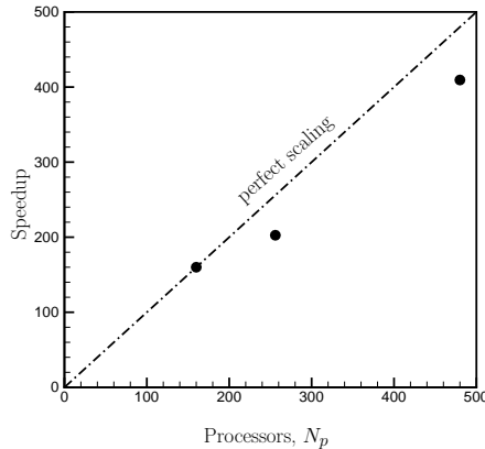
FIGURE 4. Scalability of the new CDP- \alpha code on Frost (with hypre AMG solver for pressure). Problem is the cold flow LES of the full combustor geometry with 35 M cv’s. Scaling is reported relative to the 160 processor case, which was the smallest number of Frost processors that could run this problem.
