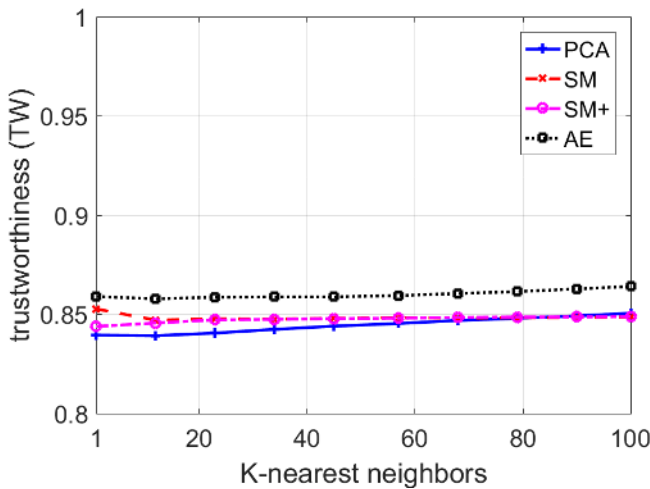
(b) Trustworthiness (TW)
