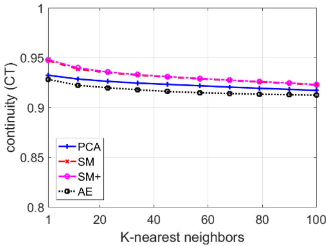
(a) Continuity (CT)
