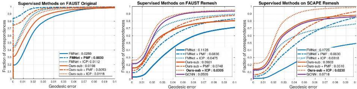
Figure 3: Quantitative evaluation of pointwise correspondences comparing our method with Supervised Methods.
