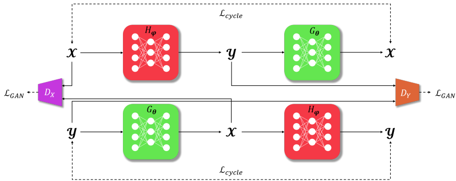
Fig. 9. Network architecture of cycleGAN. G_\theta : \mathcal{Y} \mapsto \mathcal{X}, H_\varphi : \mathcal{X} \mapsto \mathcal{Y} are the generators responsible for inter-domain mapping. D_X, D_Y are discriminators, constructing \mathcal{L}_{\text{GAN}} . GAN loss is simultaneously optimized together with \mathcal{L}_{\text{cycle}}
