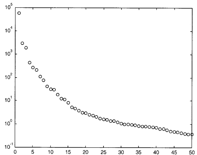
Fig. 11. Eigenvalue spectrum from PCA analysis of SEBASS scene.
