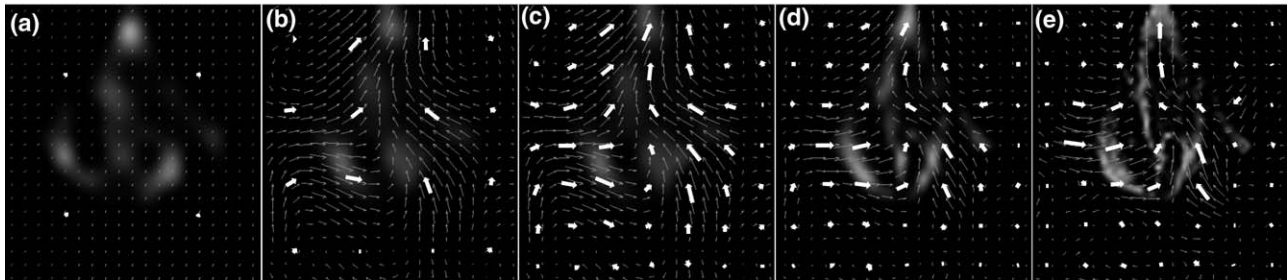
Fig. 4. Improvement of fit during optimization The graph shows a typical course of the MAD during optimization. The arrows denote a step on the deformation map pyramid ( \downarrow ) resulting in a higher deformation resolution and a step in the image pyramid ( \downarrow ) resulting in a higher image resolution. The images (a) to (e) denote the intermediate images after each of the optimization steps, as marked in their respective positions on the graph.
