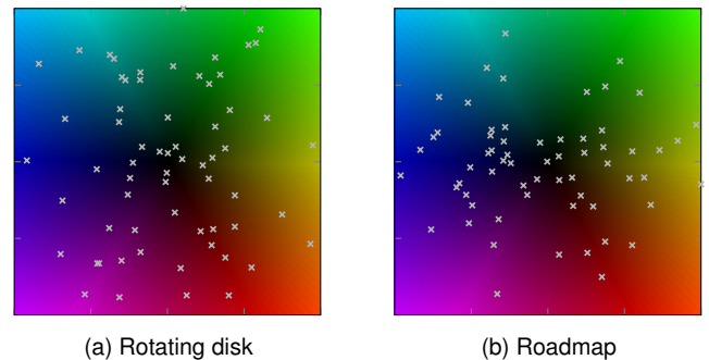
Fig. 10: MS-Conv kernels learned from real sequences in the (normalized) optical flow space.
