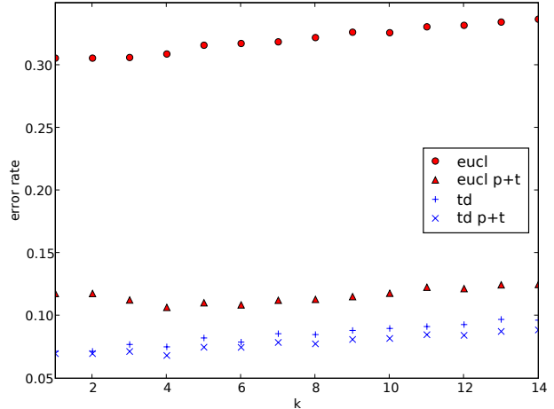
Figure 5. Error rates using k-nearest neighbors.
