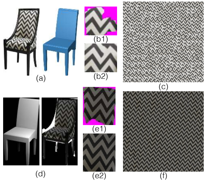
Figure 22: Effect of illumination correction. (a) input image and retrieved shape, (b1) extracted trustworthy region with patch alignment on patches cut from input image, (b2) hole filling results, (c) texture synthesis results. (d) estimated shading and illumination correction, (e1,e2) extracted trustworthy region and hole filling result, (f) final texture synthesis result.
