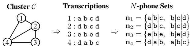
Fig. 3. Conversion of cluster nodes into groups of n -phones. The intervals under the nodes are phonetically transcribed, then separated into sets of n -phone sequences. In this example, n = 3 .
