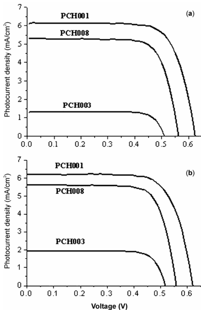
Figure 6. Current-voltage characteristics (a) M1, (b) A7117 redox electrolytes and the cell's active area 0.2 \text{ cm}^2 .
