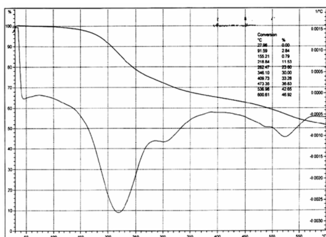
Figure 7. TG/DTG curves of PCH008 with heating rate of 10^\circ\text{C min}^{-1} under nitrogen.
