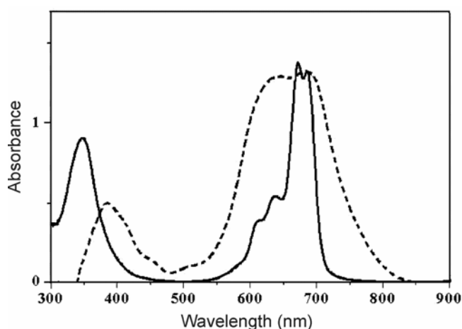
Figure 2. UV-visible absorption spectra of PCH008 (—) in ethanol and (----) adsorbed onto a 2 \mu\text{m} thick \text{TiO}_2 film.
