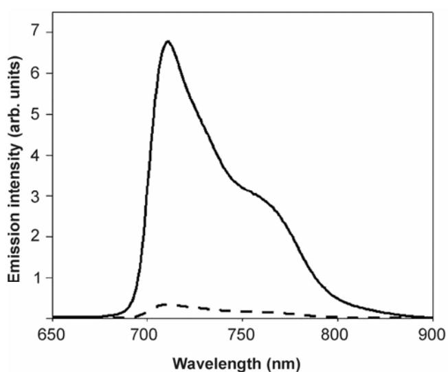
Figure 3. Fluorescence spectra of PCH008 (—) in \text{CH}_3\text{CN} and (----) adsorbed onto a 2 \mu\text{m} thick \text{TiO}_2 film. The excitation wavelength \lambda_{\text{ex}} = 686 nm.
