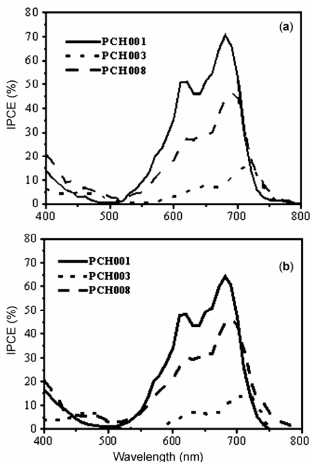
Figure 5. Photocurrent action spectra of PCH001 (—), PCH003 (.....), and PCH008 (----) with (a) M1, (b) A7117 redox electrolytes and the cell's active area 0.2 cm 2 .
