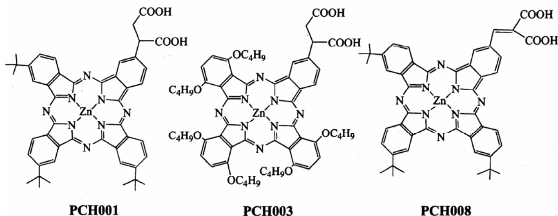
Figure 1. Molecular structures of unsymmetrical phthalocyanines used in this study.
