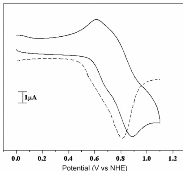
Figure 4. Cyclic (—) and differential pulse voltammograms (----) of PCH008.
