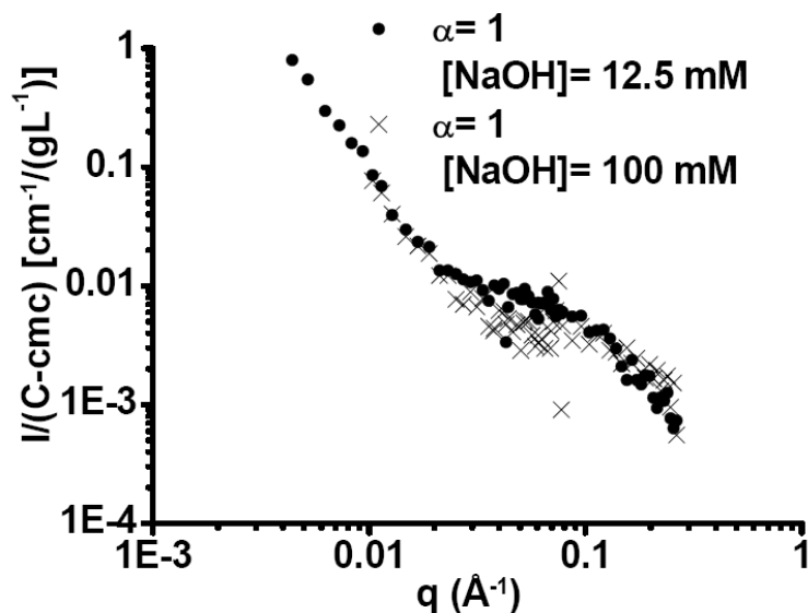
Figure 8 –SANS experiments performed on two SL solutions at \alpha= 1 but different NaOH concentrations. Data on the [NaOH]= 12.5 mM (pH= 11) system (full circles) were completed with ultra-low angle experiments ( q < 8.38 \cdot 10^{-3} \text{ \AA}^{-1} ) to confirm the increase of I(q) .
