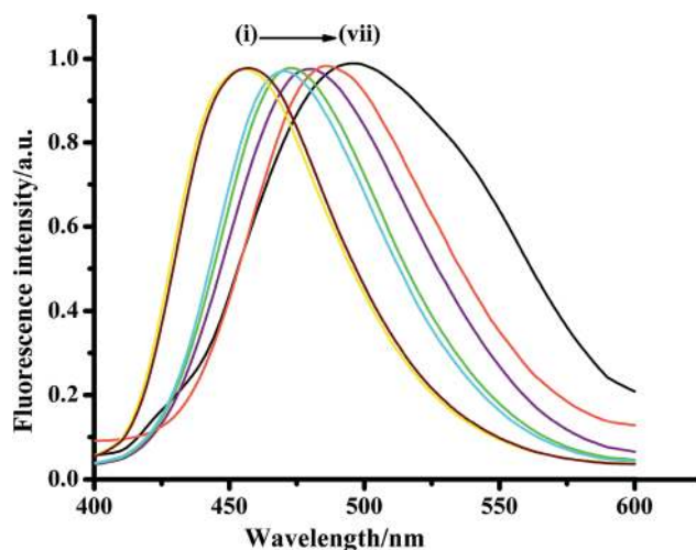
Fig. 6 Fluorescence profile of NPCP in different homogeneous solvents ( 1 \times 10^{-6} mol L -1 ; \lambda_{exc} = 370 nm). (i) n -Heptane, (ii) n -cyclohexane, (iii) dioxane, (iv) THF, (v) MeOH, (vi) ACN, (vii) water. Reproduced from ref. 78. Copyright 2015 with permission from Elsevier.
