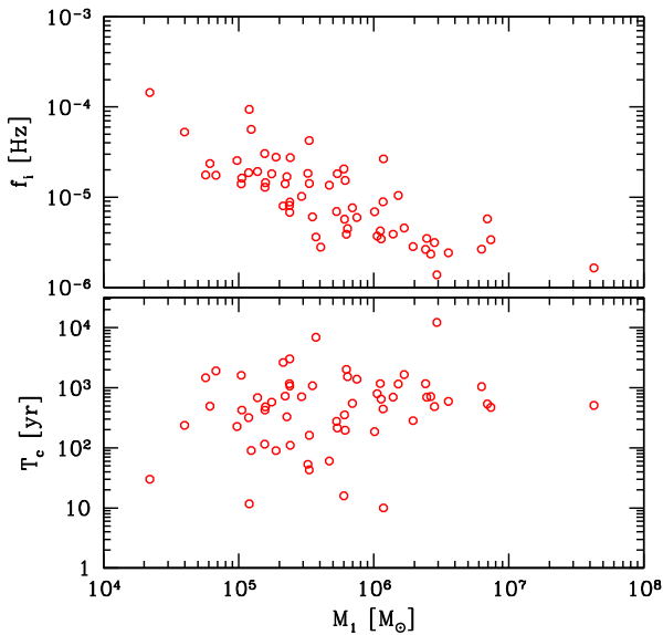
Fig. 3 Primary MBH mass vs observed frequency (top) and time to coalescence (bottom) for an illustrative local ( z < 0.5 ) inspiralling MBHBs population detected by Ares with \text{SNR} > 8 , from model HS-delayed of [49]
