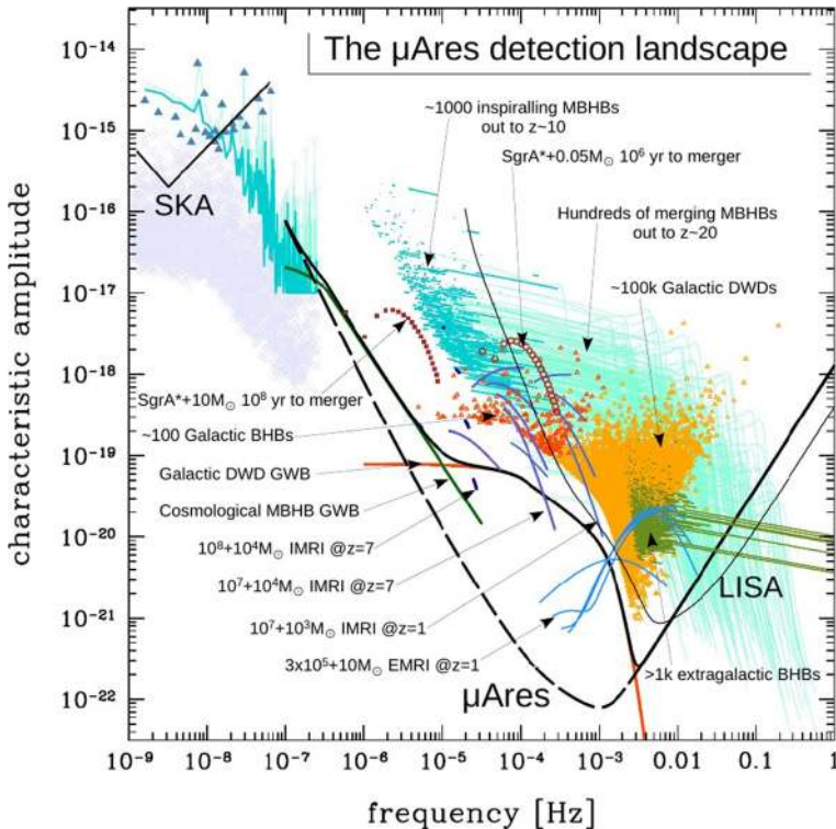
Fig. 1 Ares sky-averaged sensitivity curve (thick black curve; dashed: instrument only; solid: including astrophysical foregrounds), compared to LISA (thin solid black curve) and SKA (solid black line at the top left). Sources in the SKA portion of the figure include individual signals from a population of MBHBs (pale violet), resulting in an unresolved GWB (jagged blue line) on top of which the loudest sources can be individually resolved (dark blue triangles). The vast diversity of Ares sources is described by the labels in the figure. For all Galactic sources (including DWDs, BHBs, and objects orbiting SgrA*), the frequency drift during the observing time has been assumed to be negligible. We thus plot h\sqrt{n} , where n is the number of cycles completed over the mission lifetime, assumed to be 10 years. In this case, the signal-to-noise ratio (SNR) of the source is given by the height of its marker over the sensitivity curve. Extragalactic sources (including BHBs, MBHBs, EMRIs, and IMRIs) generally drift in frequency over the observation time. We thus plot the standard h_c = h(f^2/\dot{f}) . In this case, the SNR of the source is given by the area enclosed in between the source track and the sensitivity curve. In both cases, when multiple harmonics are present, SNR summation in quadrature applies
