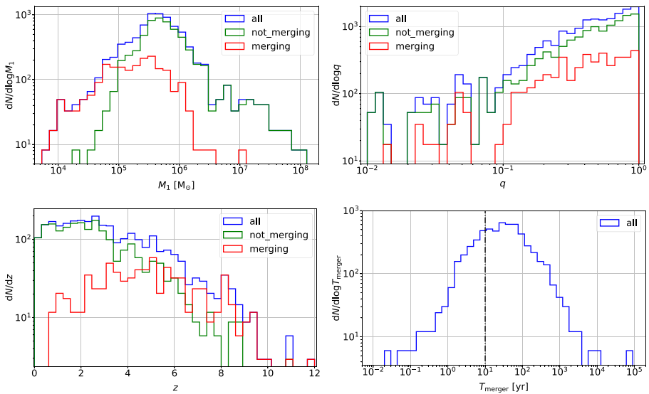
Fig. 2 Example distributions of MBHBs detected with SNR > 8 by Ares, assuming 10 years of observations. The sample comes from model HS-delayed of [49]. A total of \approx 10^3 sources are detected (blue histograms); of those, \approx 250 merge in the detector band within the mission lifetime (red histograms) and \approx 750 are observed during the adiabatic inspiral over the whole mission duration (green histograms)
