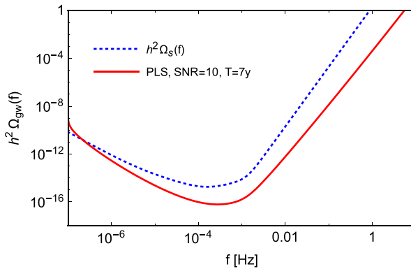
Fig. 6 Ares power law sensitivity (PLS) curves to SGWBs, obtained following the procedure outlined in [67], assuming a threshold SNR= 10 for detection. Ares reaches down to h^2\Omega_{gw} \sim 6 \times 10^{-17} at 2 \times 10^{-4} Hz, for comparison LISA is expected to get to h^2\Omega_{gw} \sim 2 \times 10^{-13} at 3 \times 10^{-3} Hz
