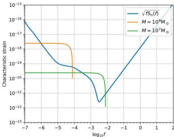
Fig. 5 Example signals from the memory effect compared to the Ares sensitivity curve. The spectrum of the signals are calculated based on the derivations done in [141]. The value of the redshift was chosen to be z = 4 . Both MBHBs were chosen to have components of equal mass. The green curve corresponds to the M = 10^7 M_\odot and the orange curve corresponds to M = 10^9 M_\odot . The values for the characteristic timescale of the memory rise is inverse proportional to the frequency at coalescence and were chosen to be \tau = 100 s and \tau = 10000 s for the green and orange curve respectively
