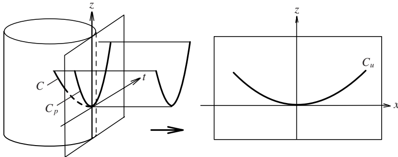
Figure 7. Curve C cut by a parabolic cylinder, with profile C_p and unwrapped curve C_u .
