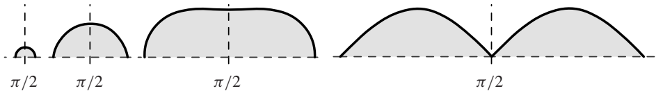
Figure 11. The unwrapped curve (upper half) is obtained by drilling a hole of unit radius through different parts of the main cylinder of the same radius. Each is symmetric about the line x = \pi/2 . The lower half (not shown) is the reflection of the upper half through the x -axis.
