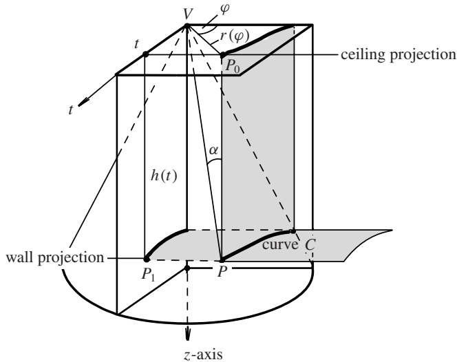
Figure 30. Relating the wall projection and ceiling projection of a curve on a right circular cone.
