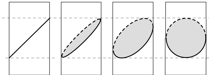
Figure 9. Various profiles of a rotating inclined ellipse. The dashed portions lie on the rear half.
