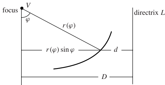
Figure 20. Diagram for deriving the polar equation of the projected conic C_0 .
