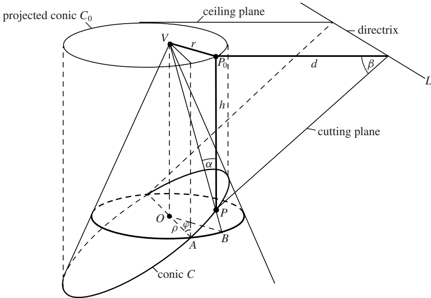
Figure 19. Diagram for proving parts (a), (b), and (c) of Theorem 7. (The ceiling plane intersects the cutting plane along the directrix L of the projected conic.)
