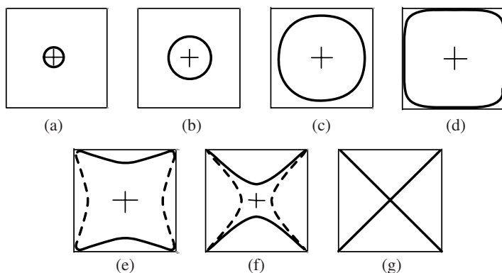
Figure 13. Profiles of the hole made by a drill of radius equal to that of the main cylinder, as the axis of the drill moves toward the axis of the main cylinder, viewed from a direction perpendicular to the axis of the drill.
