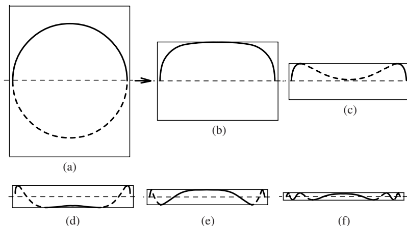
Figure 8. Rolling a circle on a transparency onto cylinders with decreasing radii.
