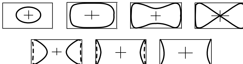
Figure 14. Profiles of the hole made by a drill of radius half that of the main cylinder, as the axis of the drill moves toward the axis of the main cylinder, viewed from a direction perpendicular to the axis of the drill.
