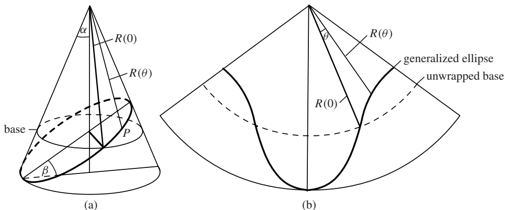
Figure 15. (a) An elliptical cross section; (b) its unwrapped image on a plane.
