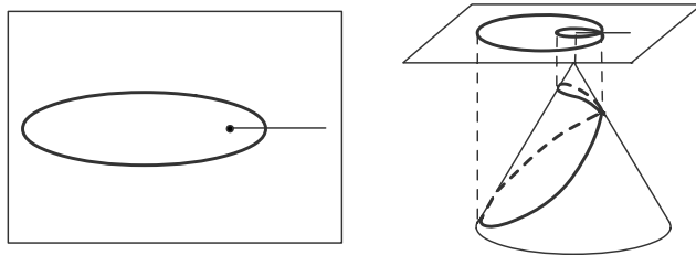
Figure 26. Generalized ellipse in Figure 25a as the ceiling projection of a curve obtained by wrapping an ellipse onto a cone with vertex angle \pi/3 to form a curve with two nonplanar loops.
