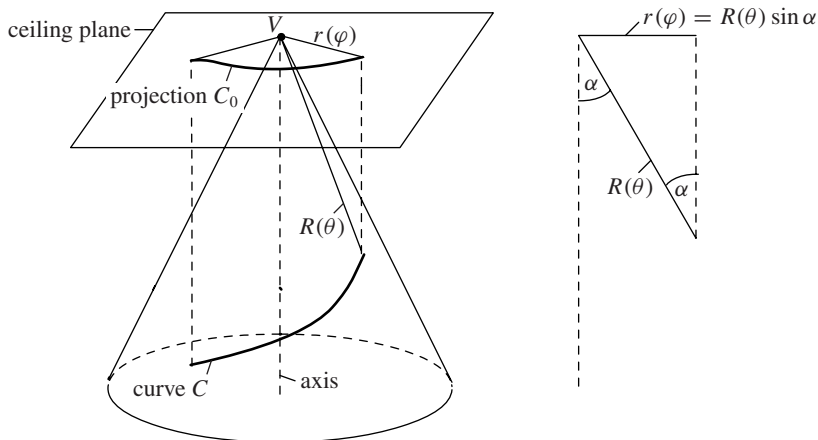
Figure 17. Curve C on the cone projects onto curve C_0 in the ceiling plane with polar equation r = r(\varphi) .
