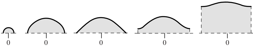
Figure 12. The unwrapped image of the upper half of a hole of variable radius drilled through the axis of the main cylinder is shown. Each is symmetric about the line x = 0 . The lower half (not shown) is the reflection of the upper half through the x -axis.
