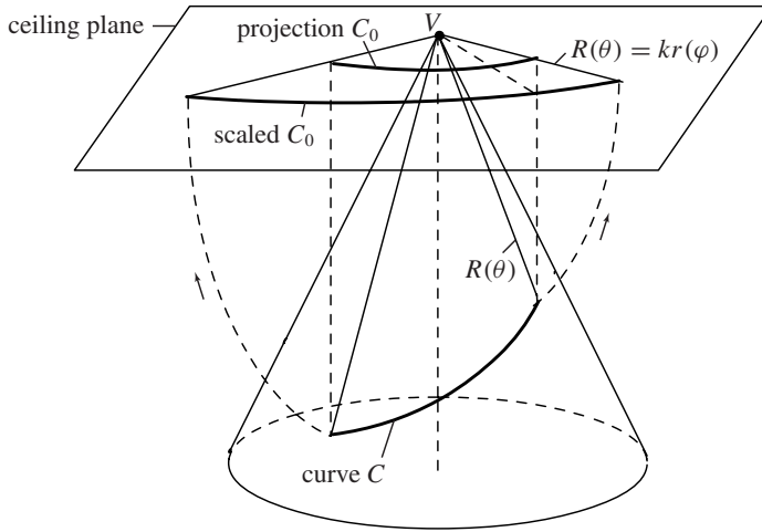
Figure 18. Umbrella transformation (20) maps curve C from the cone to a scaled version of projection C_0 .
