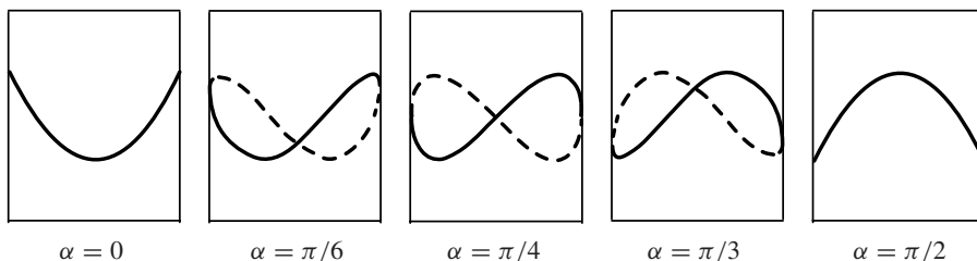
Figure 10. Rotated views of a parabolic intersection are depicted. In a perpendicular direction we see the original parabola flipped upside down.
