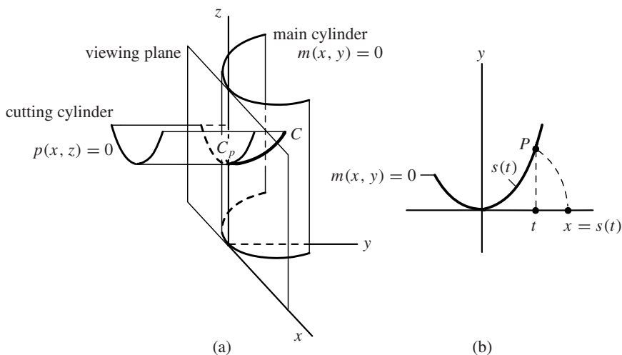
Figure 4. (a) The main cylinder and an orthogonal cutting cylinder intersect along C . (b) Point P on the horizontal profile projects onto (t, 0) and unwraps onto (s(t), 0) .
