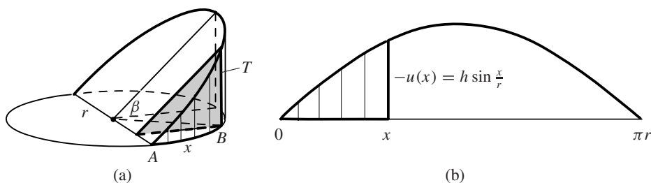
Figure 3. The circular arc AB of length x in (a) unwraps onto the line segment [0, x] in (b). The altitude of triangle T unwraps onto the height u(x) .
