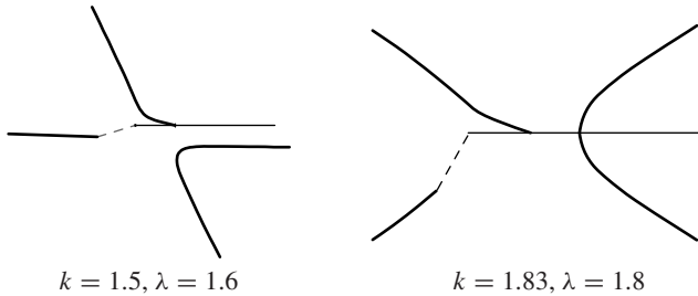
Figure 23. Generalized hyperbolas, one period. Both nappes are cut and unwrapped onto a plane.
