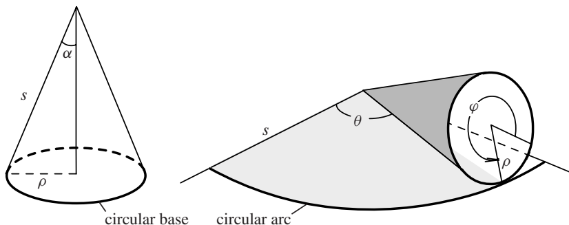
Figure 16. (a) Finite portion of a cone with slant height s ; (b) unwrapping the surface of this finite portion.
