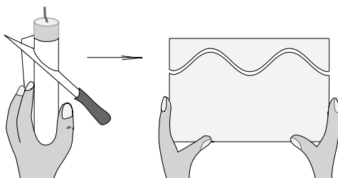
Figure 1. An elliptical cross section of a cylinder becomes sinusoidal when unwrapped.
