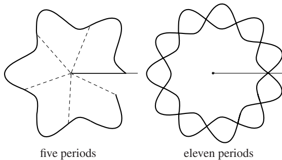
Figure 24. Second generalized ellipse from Figure 21 ( k = 5.5 , \lambda = 0.22 ), with more than one period.
