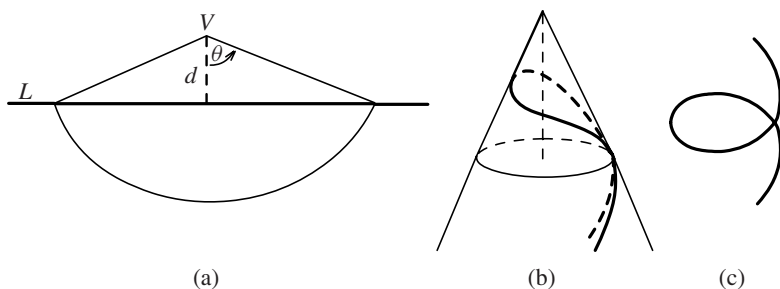
Figure 28. Line segment (a) wrapped onto a geodesic (b) on a cone, with ceiling projection (c).
