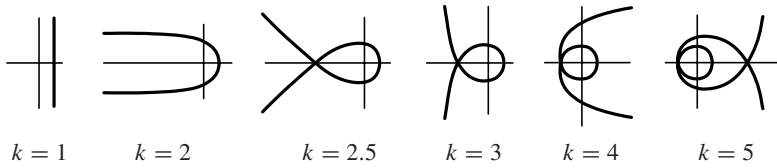
Figure 29. Ceiling projections of one line wrapped onto cones with different vertex angles ( \sin \alpha = 1/k ).
