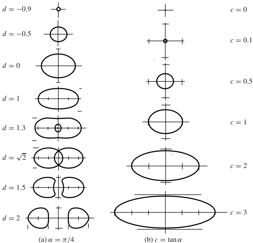
Figure 31. Snapshots of ceiling projection of a horizontal hole of radius 1 drilled through the axis. (In (a) the cone is fixed and the coordinate d varies; in (b) the drill is fixed and the vertex angle changes.)
