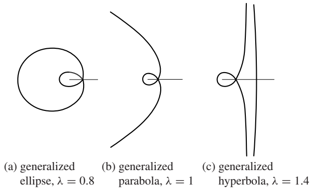
Figure 25. Generalized conics with k = 0.5 in (24). (They cannot be obtained by unwrapping a conic from a cone, but each is the ceiling projection of a conic wrapped from a plane onto a cone.)
