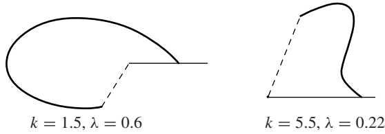
Figure 21. Generalized ellipses, one period only. (For more periods, see Figure 24.)
