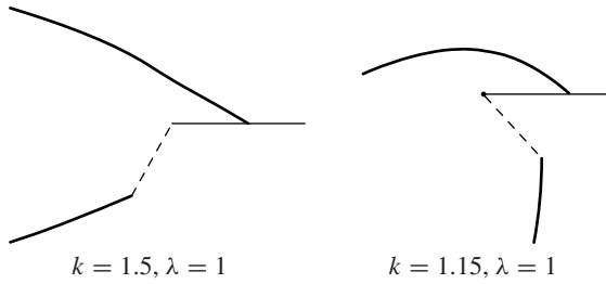
Figure 22. Generalized parabolas, one period.
