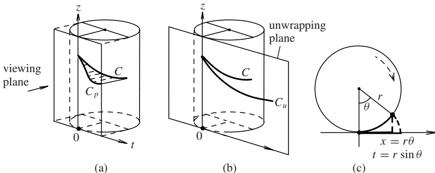
Figure 5. (a) Curve C on a circular cylinder and its horizontal profile C_p on a tangent viewing plane. (b) The unwrapped curve C_u obtained by rolling the cylinder along the unwrapping plane. (c) A point on a circle projects onto point t = r \sin \theta , but unwraps onto point x = r\theta .
