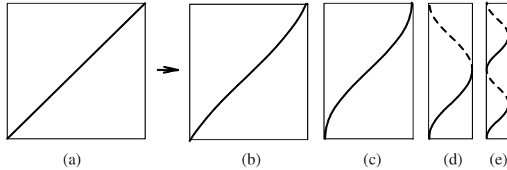
Figure 6. A line segment (a) wraps onto a geodesic. In (b)–(e) geodesic profiles (arcsine curves) are shown on cylinders of decreasing radii. The dashed curves in (d) and (e) are on the rear half of the cylinder.
