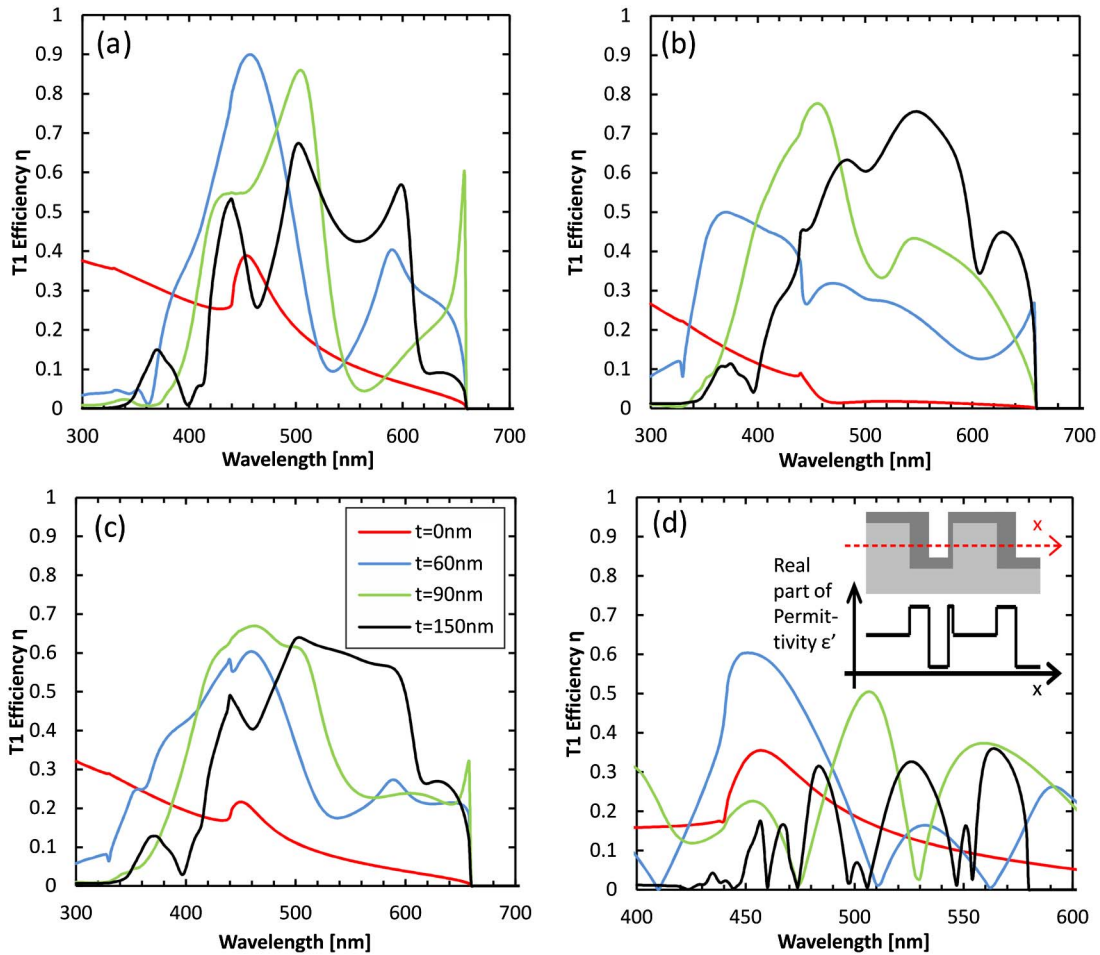
Fig. 3. Computed T1 data is plotted for increasing ZnS thicknesses t for (a) TE polarized light and (b) TM polarized light. (c) The average of the two is shown, and (d) the difference between them is shown. Inset: schematic representation of the real part of the permittivity (black line) at the lateral position indicated by the red axis in the structure sketched above.
