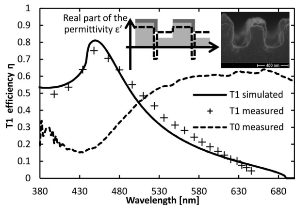
Fig. 4. Experimental T1 efficiencies (crosses) measured for perpendicularly incident TE polarized light at the individual angles plotted together with the computed data (black solid line) and zero order transmittance (dotted line). The graph exhibits efficiencies in excess of 70% for the metallized grating shown in the SEM image of the inset. The inset also depicts the real part of the permittivity along the cross section of such a structure.
