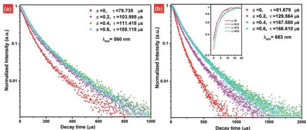
Fig. 9 Luminescence decay curves for EYBLO:xF - samples (x = 0, 0.2, 0.4 and 0.6) at the (a) 560 nm ( 4 S 3/2 → 4 I 15/2 ) and (b) 663 nm ( 4 F 9/2 → 4 I 15/2 ) emissions under the excitation of 980 nm LD; the inset shows the luminescence rise curve.
