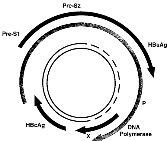
FIG. 2. Structure and organization of the HBV genome.
