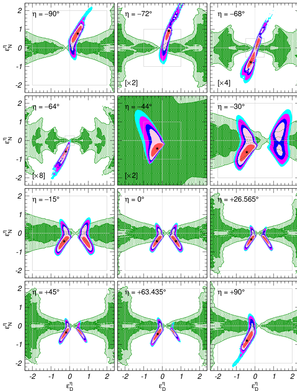
Figure 2. Two-dimensional projections of the 1\sigma , 90\% , 2\sigma , 99\% and 3\sigma CL (2 dof) allowed regions from the analysis of solar and KamLAND data in the presence of non-standard matter potential for the matter potential parameters (\varepsilon_D^\eta, \varepsilon_N^\eta) , for \sin^2 \theta_{13} = 0.022 and after marginalizing over the oscillation parameters. The best-fit point is marked with a star. The results are shown for fixed values of the NSI quark coupling parameter \eta . The panels with a scale factor “[ \times N ]” in their lower-left corner have been “zoomed-out” by such factor with respect to the standard axis ranges, hence the grey square drawn in each panel always corresponds to \max(|\varepsilon_D^\eta|, |\varepsilon_N^\eta|) = 2 and has the same size in all the panels. For illustration we also show as shaded green areas the 90\% and 3\sigma CL allowed regions from the analysis of the atmospheric and LBL data. Note that, as a consequence of the periodicity of \eta , the regions in the first ( \eta = -90^\circ ) and last ( \eta = +90^\circ ) panels are identical up to an overall sign flip.
