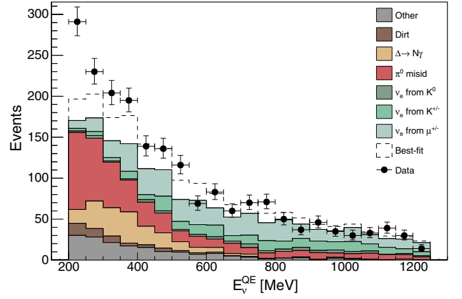
FIG. 25. The MiniBooNE neutrino mode E_\nu^{\text{QE}} distributions, corresponding to the total 18.75 \times 10^{20} POT data in neutrino mode in the 200 < E_\nu^{\text{QE}} < 1250 MeV energy range, for \nu_e CCQE data (points with statistical errors) and background (histogram) with radius less than 4 m. The dashed histogram shows the best fit to the neutrino-mode data assuming two-neutrino oscillations.
