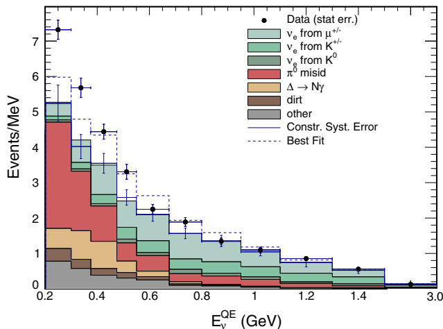
FIG. 9. The MiniBooNE neutrino mode E_\nu^{\text{QE}} distributions, corresponding to the total 18.75 \times 10^{20} POT data in the 200 < E_\nu^{\text{QE}} < 3000 MeV energy range, for \nu_e CCQE data (points with statistical errors) and predicted backgrounds (colored histograms). The constrained background is shown as additional points with systematic error bars. The dashed histogram shows the best fit to the neutrino-mode data assuming two-neutrino oscillations. The last bin is for the energy interval from 1500–3000 MeV.
