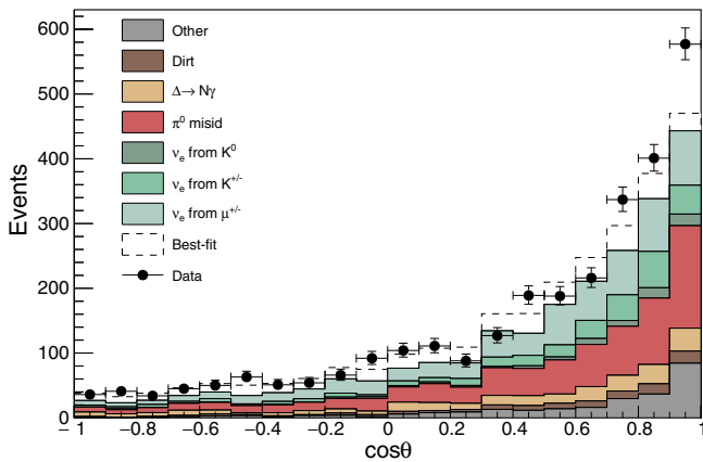
FIG. 8. The MiniBooNE neutrino mode \cos\theta distributions, corresponding to the total 18.75 \times 10^{20} POT data in the 200 < E_\nu^{\text{QE}} < 1250 MeV energy range, for \nu_e CCQE data (points with statistical errors) and background (colored histogram). The dashed histogram shows the best fit to the neutrino-mode data assuming two-neutrino oscillations.
