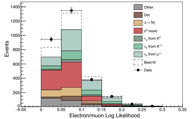
FIG. 2. The MiniBooNE neutrino mode electron-muon particle identification distributions, corresponding to the total 18.75 \times 10^{20} POT data in the 200 < E_\nu^{\text{QE}} < 1250 MeV energy range, for \nu_e CCQE data (points with statistical errors) and background (colored histogram). The dashed histogram shows the best fit to the neutrino-mode data assuming two-neutrino oscillations.
