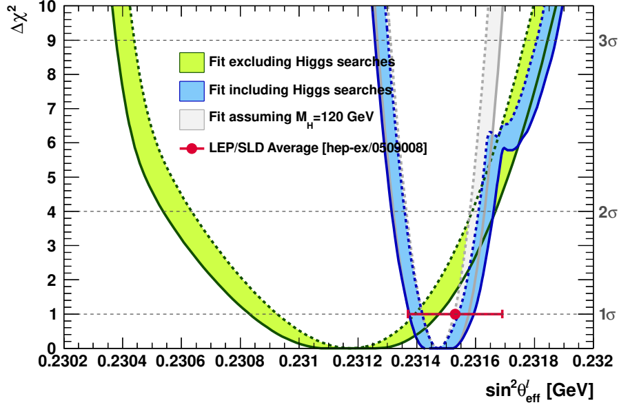
Figure 8: Indirect determination of the effective weak mixing angle: profile of \Delta\chi^2 versus \sin^2\theta_{\text{eff}}^\ell for the complete fit (blue shaded curve) and the standard fit (green shaded curve). In both fits all measurements with a direct relationship to \sin^2\theta_{\text{eff}}^\ell (e.g. the asymmetry parameters) are not included, and only the measured or determined values of m_t , M_W , \overline{m}_c , \overline{m}_b , \Delta\alpha_{\text{had}}^{(5)}(M_Z^2) and \alpha_s(M_Z^2) are used. The widths of the bands indicate the size of the cumulative theoretical uncertainty in the fit. The LEP/SLD average for \sin^2\theta_{\text{eff}}^\ell as derived directly from the asymmetry measurements is indicated by the dot with 1\sigma error bar. The light shaded curve shows the constraint one would obtain for a hypothetical Higgs discovery at 120 GeV (with negligible error on M_H ).
