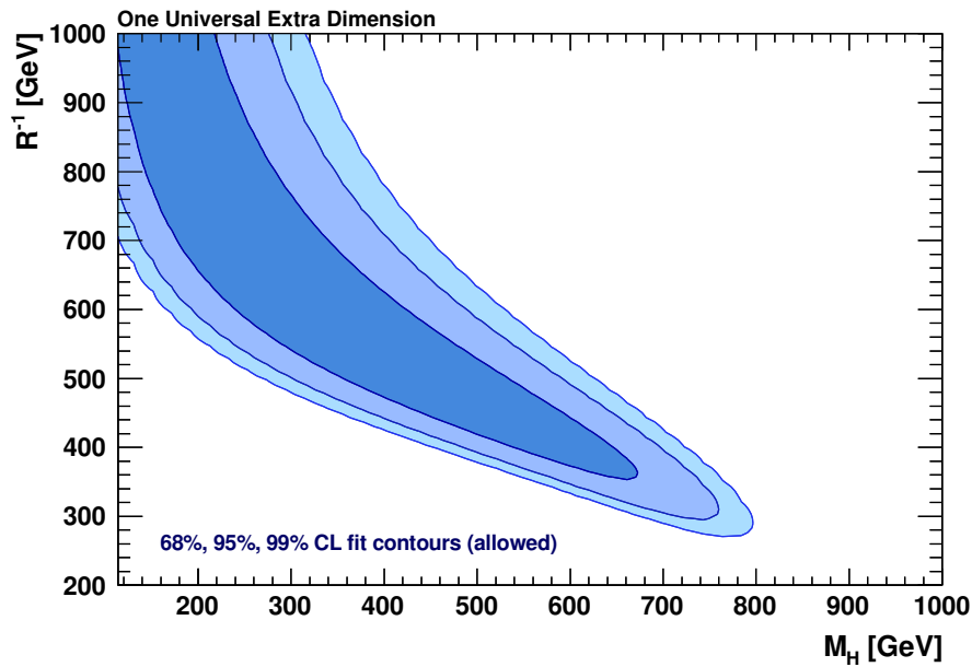
Figure 25: Constraints in the model with one universal extra dimension. Shown are the 68%, 95%, and 99% CL allowed fit contours in the (M_H, R^{-1}) plane.
