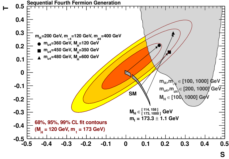
Figure 13: Oblique parameters in a model with a fourth fermion generation. Shown are the S, T fit results (leaving U free) compared with the prediction from the SM (dark grey) and the sequential fourth generation model with vanishing flavour mixing (light grey). The symbols illustrate the predictions for three example settings of the parameters m_{U_4}, m_{d_4}, m_{\nu_4}, m_{l_4} and M_H . The light grey area is obtained by varying the free mass parameters in the ranges indicated in the figure.
