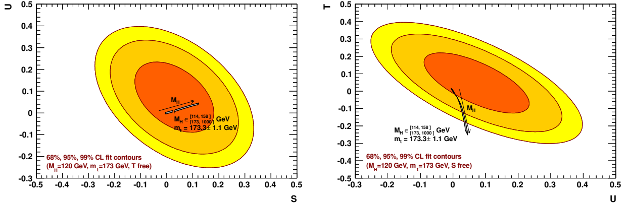
Figure 12: Experimental constraints on the S , U (left) and U , T parameters (right) with respect to the SM reference represented by M_{H,\text{ref}} = 120 GeV, m_{t,\text{ref}} = 173 GeV and the corresponding best fit values for the remaining SM parameters. Shown are the 68%, 95% and 99% CL allowed regions, where the third parameter is left unconstrained. The narrow dark grey bands illustrate the SM prediction for varying M_H and m_t values (see figures for the ranges used).
