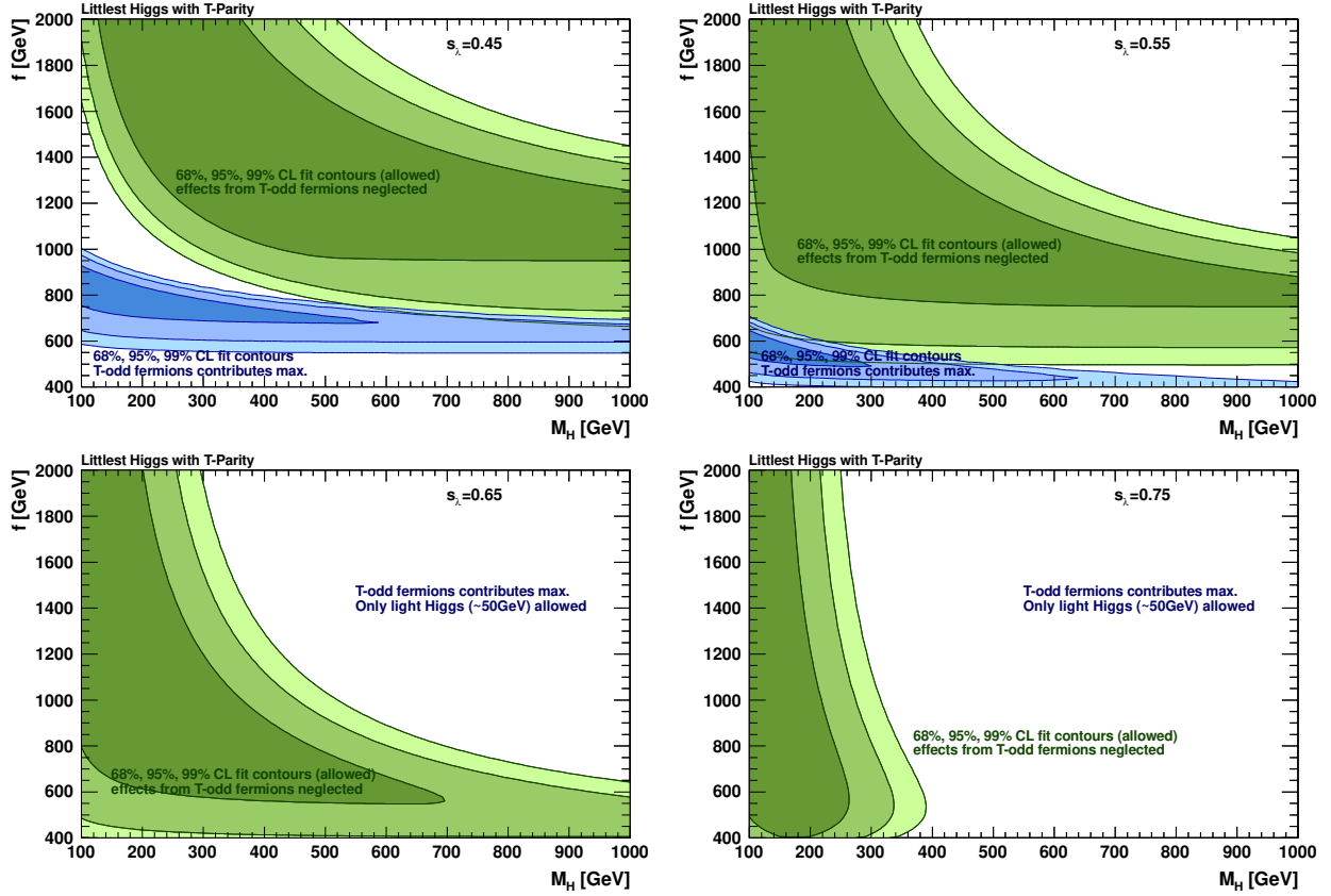
Figure 21: Constraints in the littlest Higgs model with T -parity conservation. Shown are the 68%, 95%, and 99% CL allowed fit contours in the (M_H, f) plane for fixed s_\chi values of 0.45, 0.55, 0.65 and 0.75 (top left to bottom right) when neglecting the effects from the T -odd fermions (green), and when using the bound (31) (blue, only shown for s_\chi = 0.45 and 0.55).
