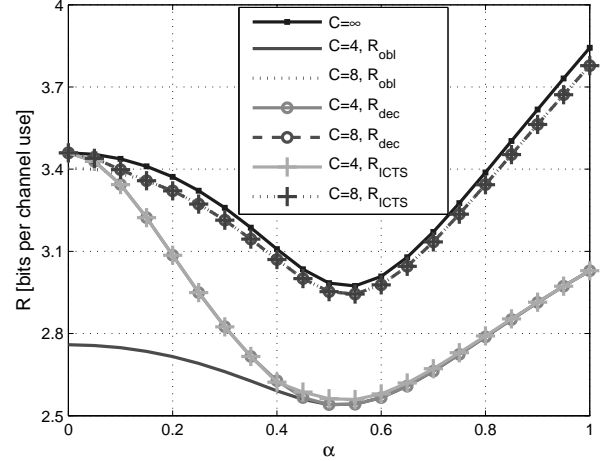
Fig. 1. The achievable rates R_{obl} , R_{dec} and R_{ICTS} are plotted as functions of the inter-cell interference \alpha for C = 4, 8, \infty and user SNR P = 10 [dB].
