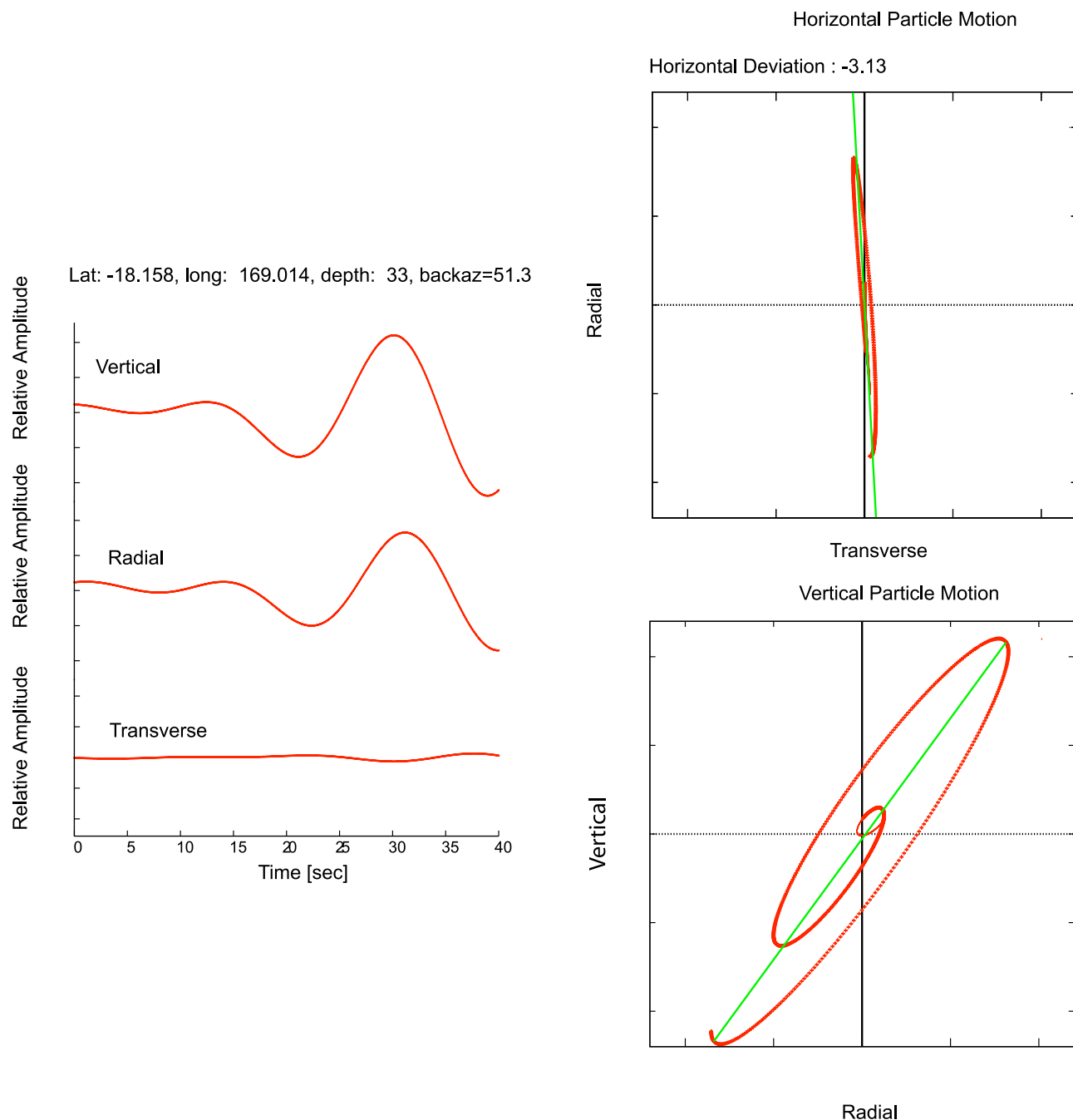
Figure 1. Example of P_{\text{pol}} measurement obtained at CAN for an earthquake occurring in the Vanuatu region; year 2000, day 060, at latitude 18.158^{\circ}\text{S} , longitude 169.014^{\circ} , depth 33 km. The epicentral distance is 24.7^{\circ} and the back azimuth 51.3^{\circ} . The departure of the actual polarization of the P wave in the horizontal plane from the radial direction (horizontal deviation of polarization: -3.13^{\circ} ) is illustrated.
