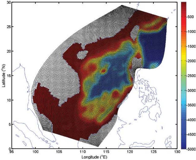
Figure 1. Model domain and grids, as well as bathymetry.
