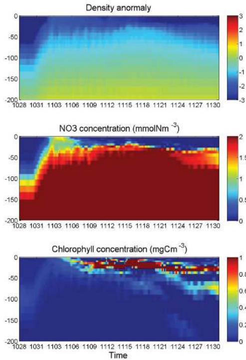
Figure 9. Profiles of chlorophyll a and nitrate concentration at the location (18.66°N, 115.89°E), shown in Figure 7 in the typhoon wake from October 28 to November 30, 2006.
