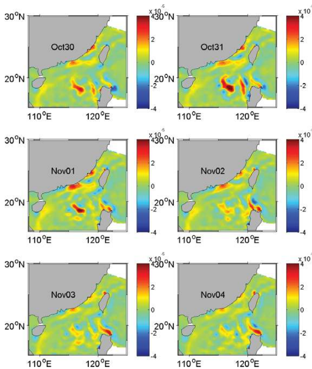
Figure 5. Surface vorticity from October 30 to November 4, 2006.
