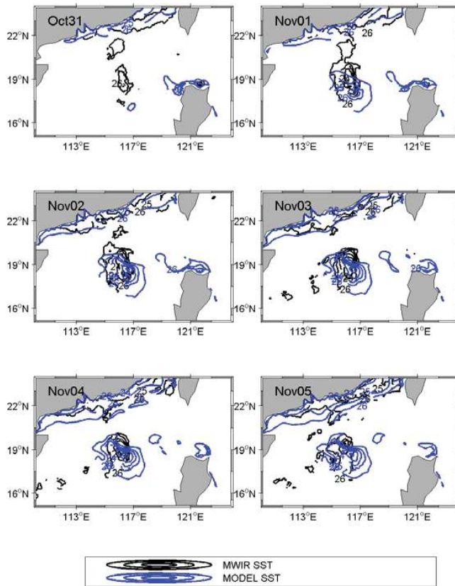
Figure 4. Isotherms of SST in the typhoon wake (unit: ^{\circ}\text{C} ) from October 31 to November 5, 2006 (with the black lines showing the MWIR OI SSTs and blue lines showing the simulated SSTs).
