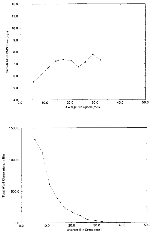
FIG. 9. Same as Fig. 8 except for WVWV produced by CIMSS from the 7.0- \mu\text{m} channel.
