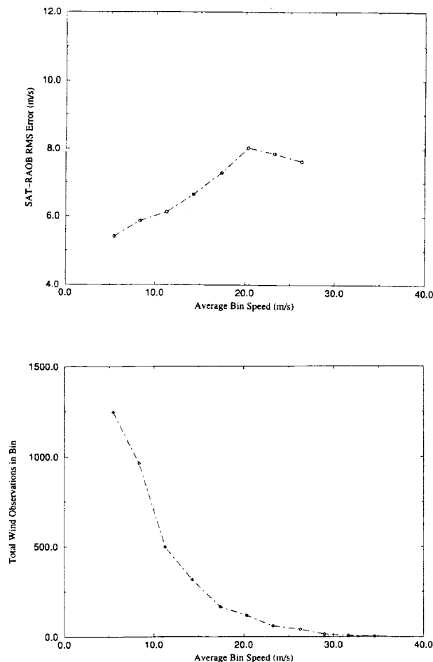
FIG. 10. Same as Fig. 8 except for WVV produced by CIMSS from the 7.3- \mu m channel.
