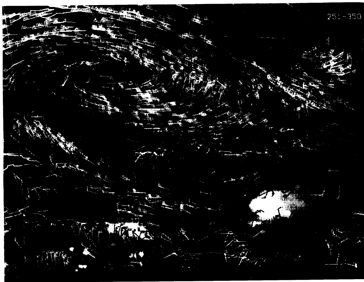
FIG. 5. High-density GOES -8 water vapor winds (6.7- \mu\text{m} channel) during Tropical Storm Pablo (lower right) on 7 October 1995. Vectors are in kt and colors refer to assigned heights (mb) with the legend in the upper right-hand corner.
