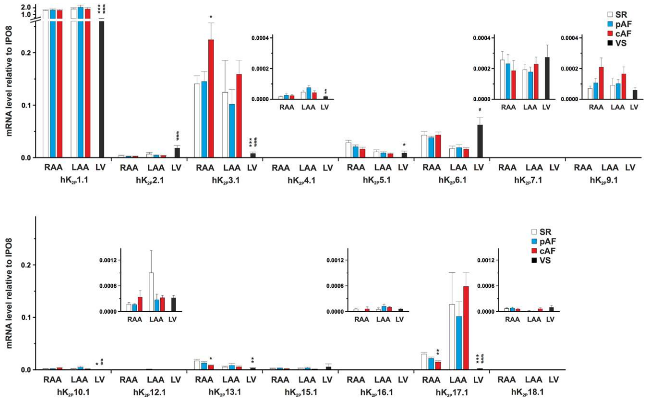
Figure 1. Cardiac expression and remodeling of K_{2p} channel mRNA in patients with sinus rhythm (SR), paroxysmal atrial fibrillation (pAF), and chronic atrial fibrillation (cAF). Ventricular samples (VS) were analyzed for comparison. Insets represent selective enlargements to visualize transcript levels of subunits with low expression. Note that the function of K_{2p}1.1 , K_{2p}7.1 , K_{2p}12.1 , and K_{2p}15.1 protein has not been unequivocally established to date. Data are expressed as mean \pm SEM arbitrary units normalized to IPO8. IPO8 indicates importin 8; LAA, left atrial appendage; LV, left ventricle; and RAA, right atrial appendage. * P <0.05, ** P <0.01, *** P <0.001 vs RAA/SR; # P <0.05, ## P <0.01, ### P <0.001 vs LAA/SR.
