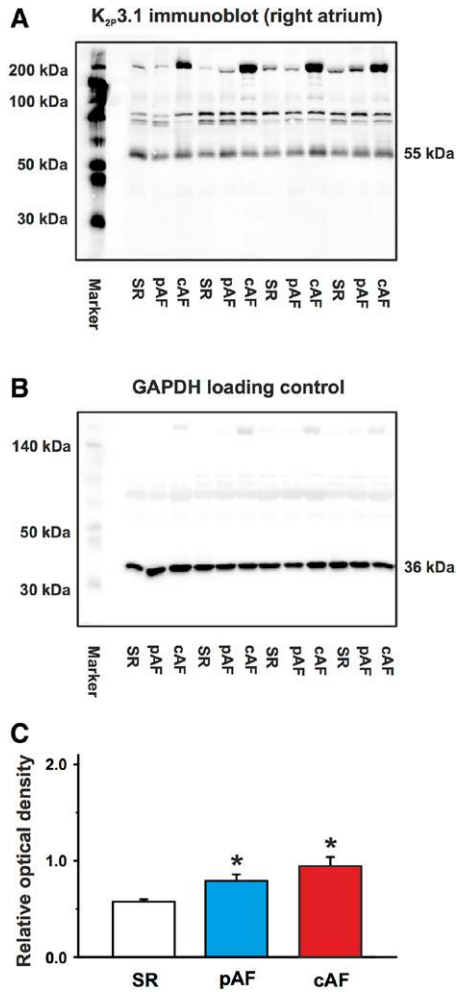
Figure 3. Western blot analysis of K_{2p}3.1 protein in human right atrium. A , Representative immunoblots obtained from patients in sinus rhythm (SR), paroxysmal atrial fibrillation (pAF), or chronic atrial fibrillation (cAF) probed with anti- K_{2p}3.1 antibodies. B , Anti-GAPDH antibodies were applied to quantify protein load. C , Mean \pm SEM optical density values normalized to GAPDH expression of indicated patient groups ( n=4 subjects per group; * P<0.05 vs SR).
