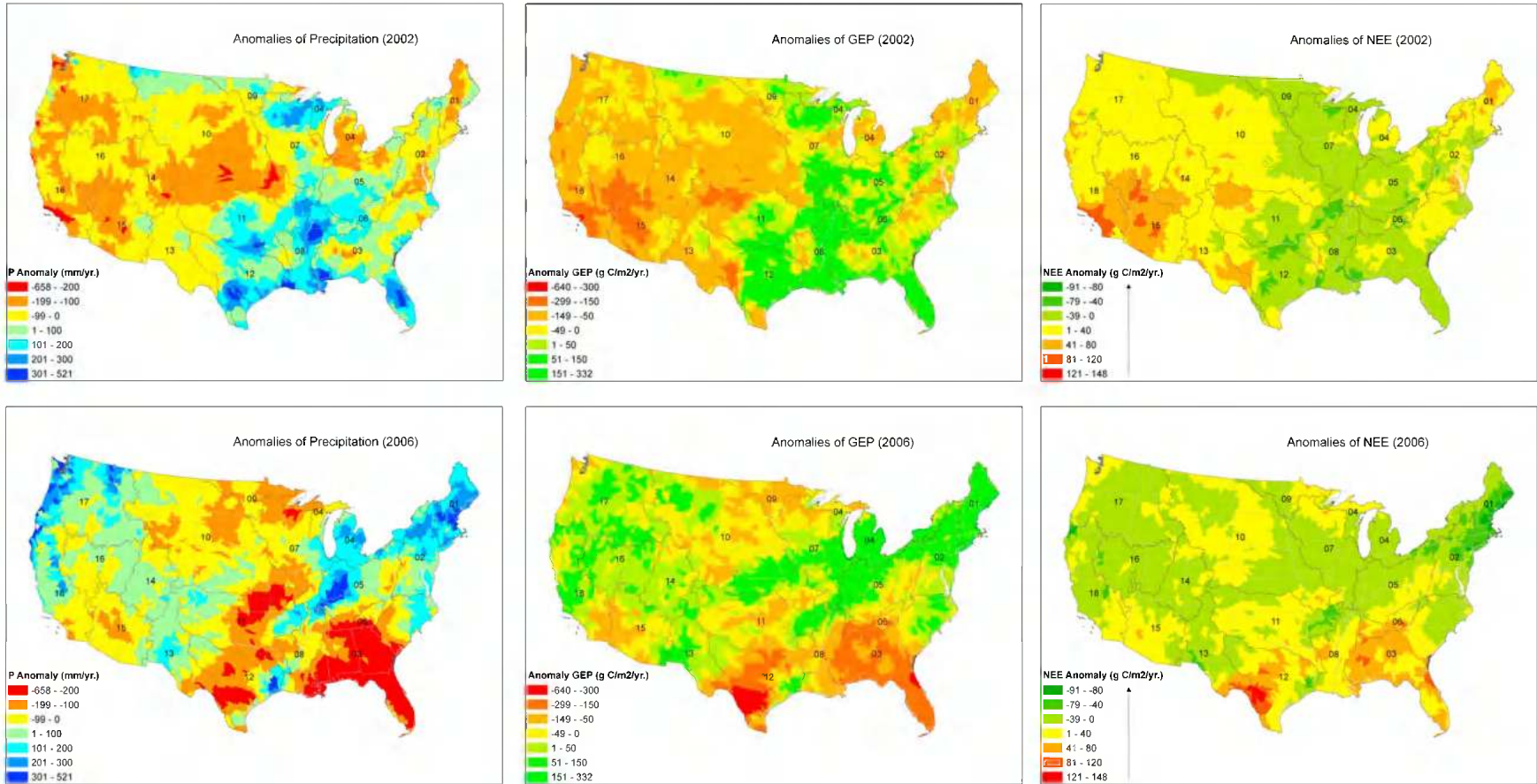
Figure 13. Anomalies of annual precipitation relative to the 48 year period 1960–2007 taken from the PRISM climate database and anomalies of GEP and NEE relative the 6 year mean in 2002 and 2006, showing impacts of server droughts on ecosystem fluxes. The arrows indicate an increase of carbon sequestration potential (more native in NEE).
