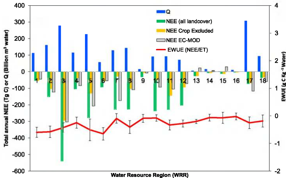
Figure 11. Summary of modeled mean annual water yield, carbon gain or loss expressed as Q (billion \text{m}^3 \text{ yr}^{-1} ) and NEE ( \text{Tg yr}^{-1} ), and ecosystem water use efficiency (EWUE) ( \text{NEE/ET} , \text{g C kg}^{-1} \text{ H}_2\text{O} ) by water resource region (WRR).
