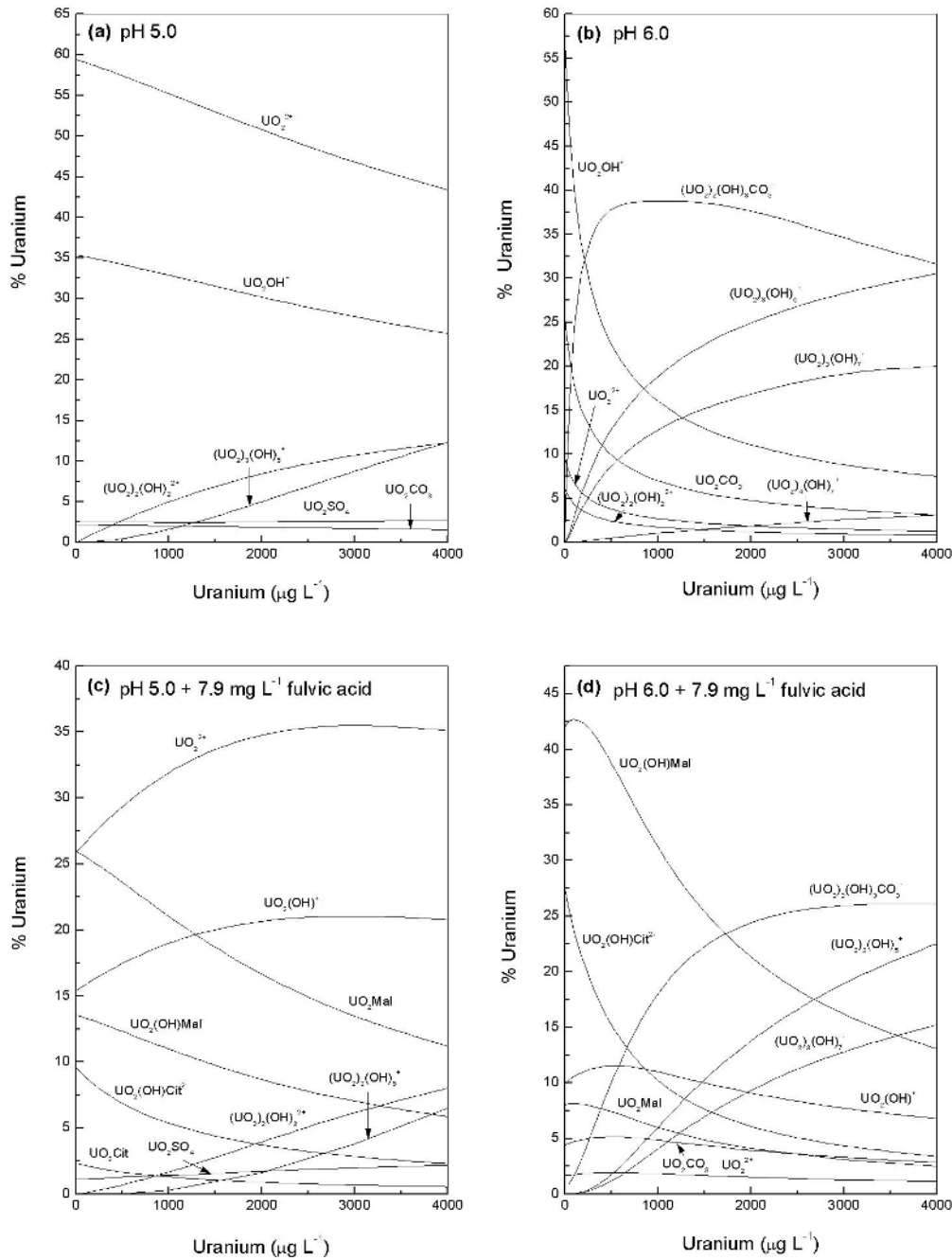
FIGURE 4. Predicted speciation (% distribution) of U in synthetic Magela Creek water at (a) pH 5.0 without model fulvic acid (FA); (b) pH 6 without model FA; (c) pH 5 with 7.9 mg l -1 model FA; and (d) pH 6 with 7.9 mg l -1 model FA.
