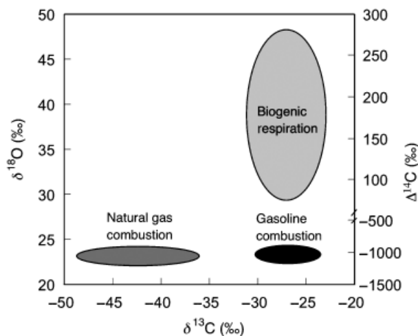
Fig. 4 Common ranges of the stable carbon isotope composition ( \delta^{13}C relative to the V-PDB Standard), oxygen isotope composition ( \delta^{18}O relative to the V-SMOW Standard) and radiocarbon composition ( \Delta^{14}C relative to the oxalic acid standard) of urban CO 2 sources.
