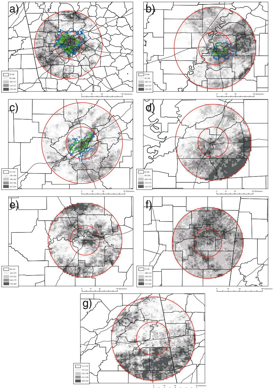
Fig. 1 Frequency of June–August medium and high reflectivity days, or total days \geq 40 dBZ in each 2-km grid cell, for the 10-year period of record for (a) Atlanta, (b) Memphis, (c) Birmingham, (d) Jackson, (e) Montgomery, (f) Starkville control, and (g) Heflin control. Red circles correspond to urban–rural buffers outlined in Table 1. For (a–c), the blue (green) lines represent NLCD (USGS) urban delineations
