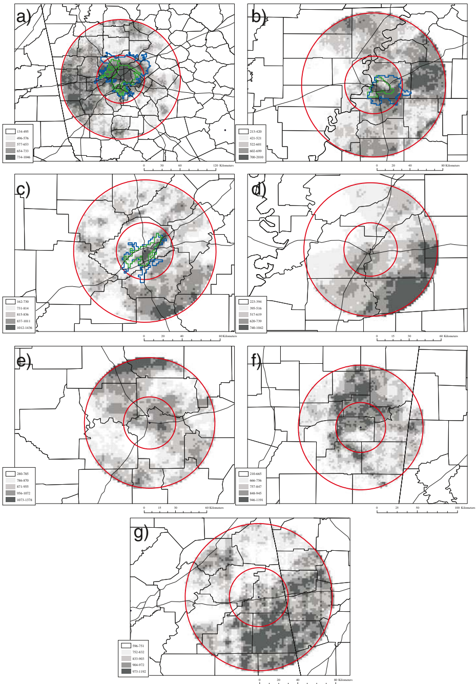
Fig. 2 As in Fig. 1, except frequency of June–August medium and high reflectivity occurrences, or total number of 5-minute occurrences \geq 40 dBZ in each 2-km grid cell, for the 10-year period of record
