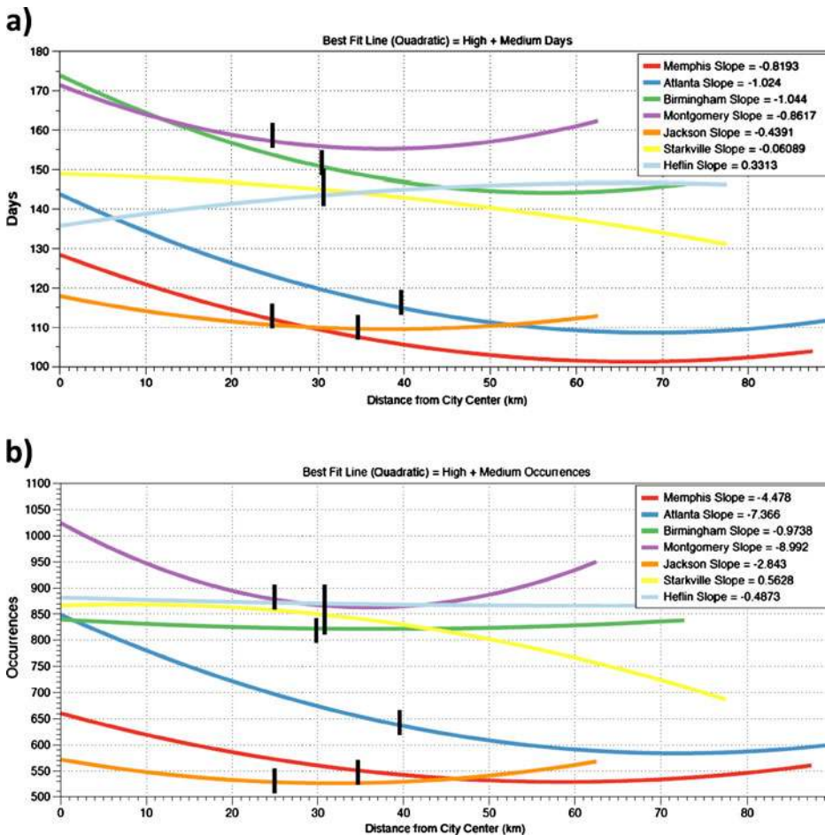
Fig. 4 Quadratic line fits representing the relative frequency of (a) total days \geq 40 dBZ and (b) total number of 5-minute occurrences \geq 40 dBZ versus distance from city center for the seven domains examined. Various urban-rural buffers used (see Table 1) are represented by black line segments
