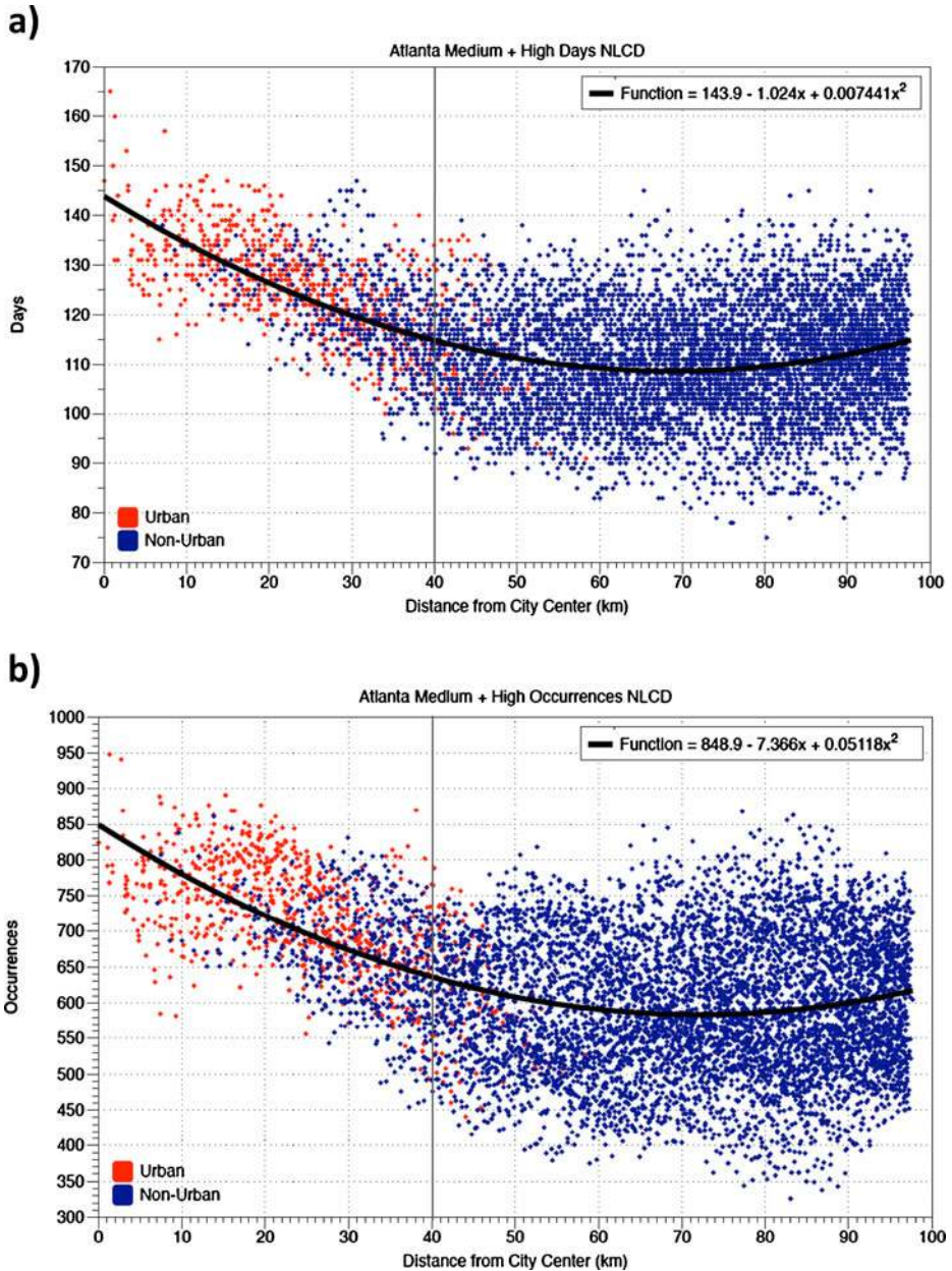
Fig. 3 Quadratic line fits and associated scatterplots representing the frequency of (a) total days \geq 40 dBZ and (b) total number of 5-minute occurrences \geq 40 dBZ for each 2-km grid cell versus distance from city center in the Atlanta domain for the 10-year, June–August period of record. NLCD urban delineated cells are colored red, whereas non-urban cells are blue. The 40-km urban buffer for Atlanta is represented as solid line emanating from the x axis
