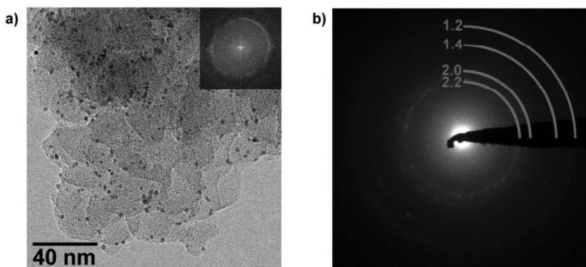
33 Figure 6. Electron microscopy analyses of the urea- CN_x after 100+ h photocatalysis: a) TEM 34 and the FFT with the quarter circle indicating a d -spacing of 11 Å (inset); b) electron 35 diffraction pattern showing the d -spacings in Å of Pt. 36 37 38 39 40 41 42 43 44 45 46 47 48 49 50 51 52 53 54 55 56 57 58 59 60 61 62 63 64 65
