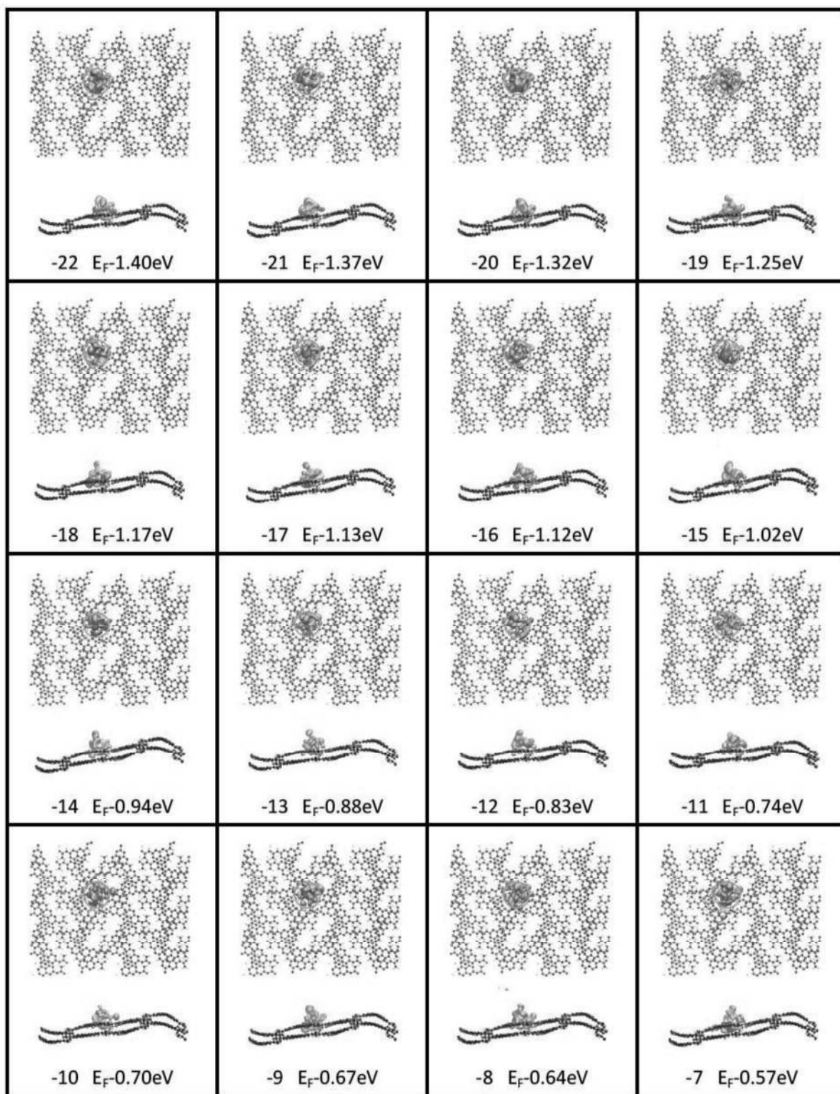
Figure S12 Part 2 of the orbital plots of \text{Pt}_{13}\text{-urea-CN}_x from just below the valence band maximum (VBM) to just above the conduction band minimum (CBM)
