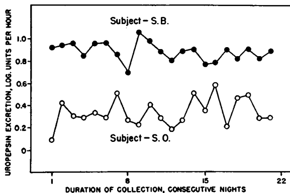
FIG. 4. UROPEPSIN EXCRETION PATTERNS OF TWO SUBJECTS
