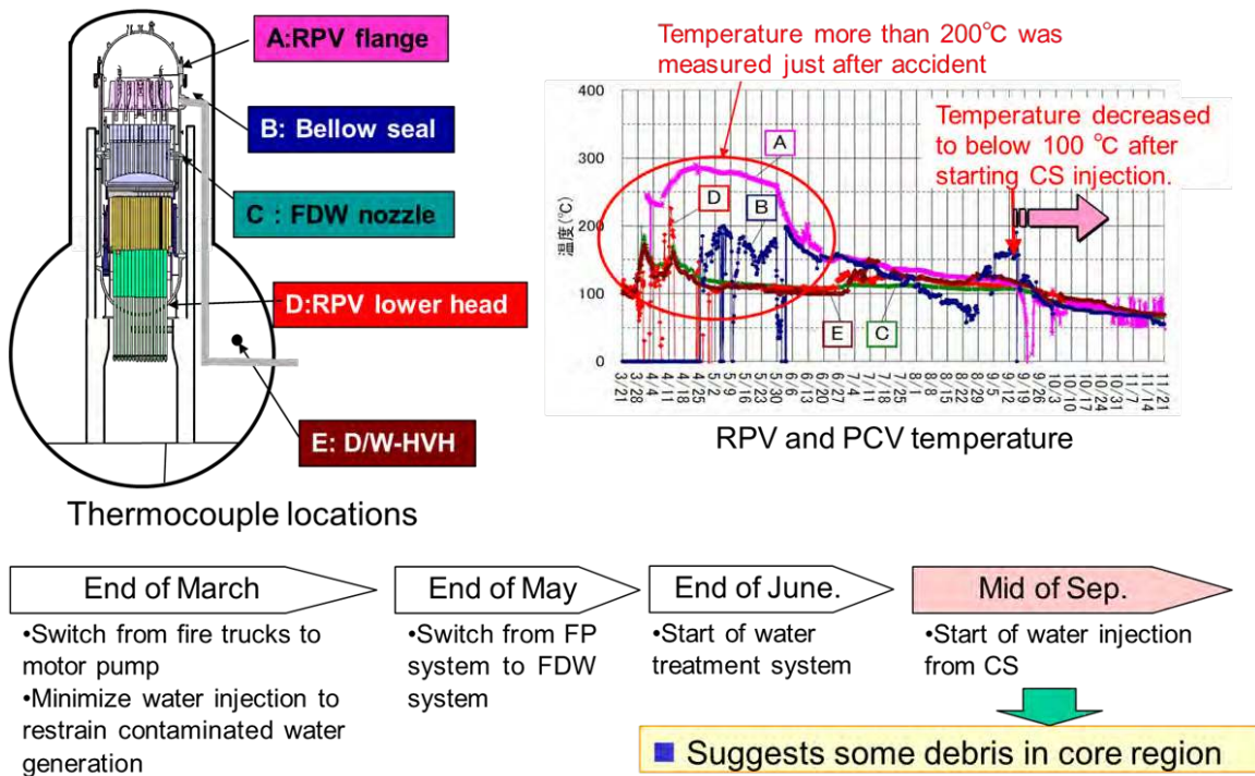
Figure 21. RPV temperature measurements for 1F2 following the accident. (Courtesy of TEPCO [10])
