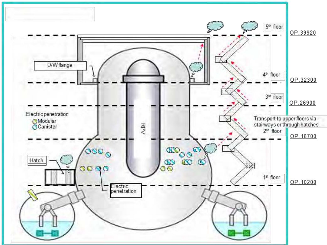
Figure 35. Inferred leakage paths; flow paths differ from 1F1 and 1F3 due to system configuration. (Courtesy of TEPCO, [131])
