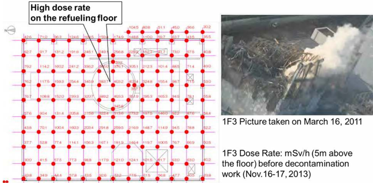
Figure 11. 1F3 radiation survey (value in mSv/hr measured on November 16-17, 2013 at 5 m above the floor at points shown on red grid) and photograph taken on March 16, 2011 (Courtesy of TEPCO [10,12])
