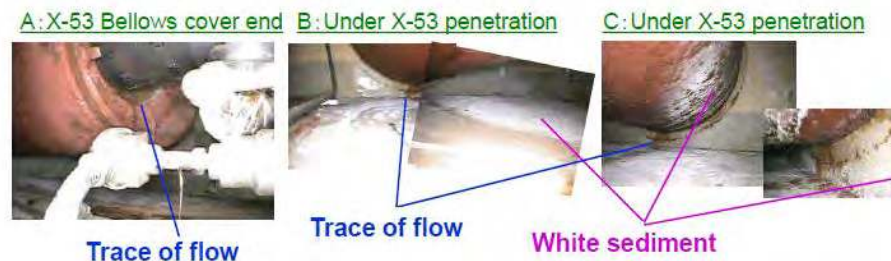
Figure 29. Photographs of leakage location and sediment. (Courtesy of TEPCO [15])
