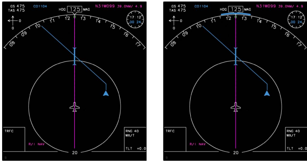
Figure 8. “False Negative” Situation Occurring with Current Display (left) and Re-designed Display Incorporating Intent-based CP Logic (right).
