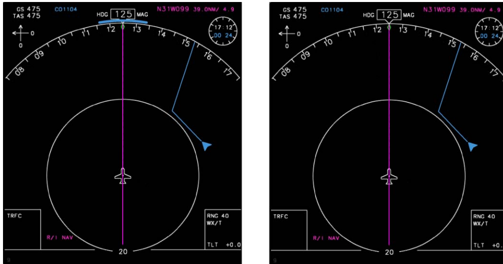
Figure 9. “False Positive” Situation Occurring with Current Display (left) and Re-designed Display Incorporating Intent-based CP Logic (right).
