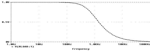
Figure 9 Frequency domain behavior of best circuit of generation 0.
