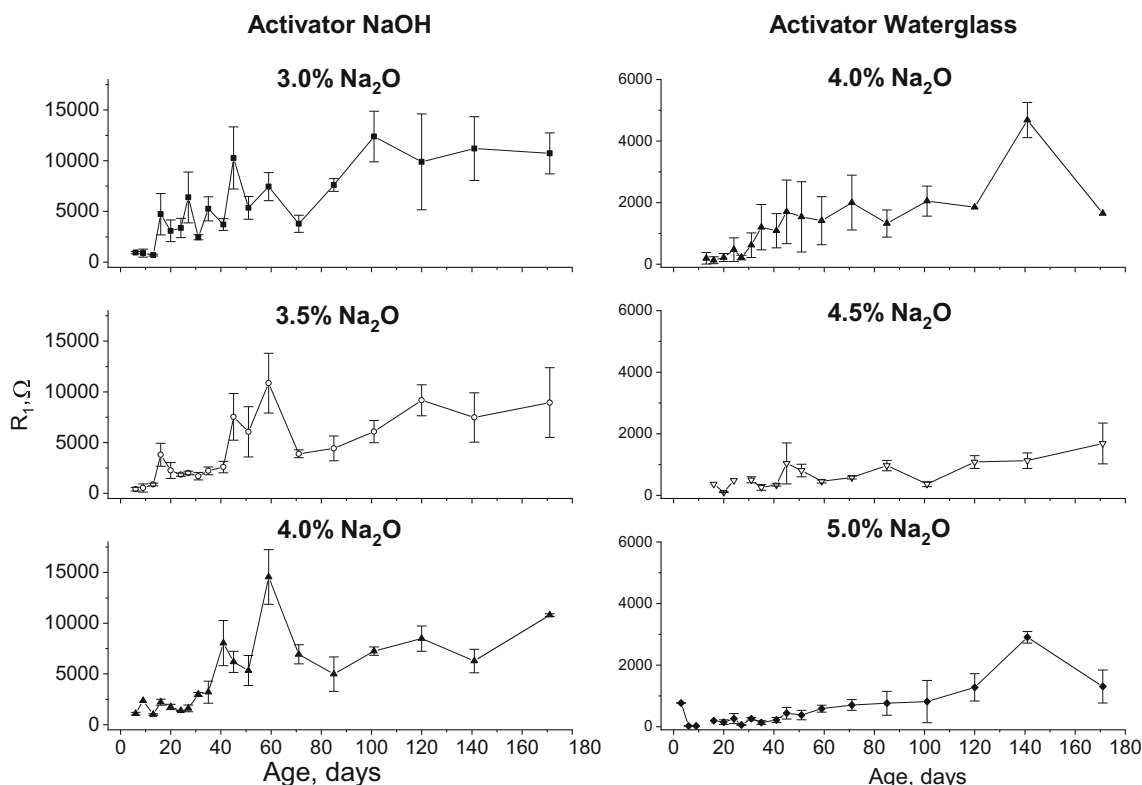
Fig. 7 Time evolution of the resistance R_1 as a function of activator and sodium oxide content
